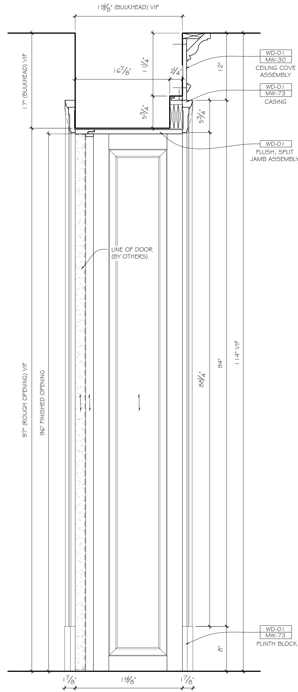
3 SECTION 1.06 SCALE: 1/2" = 12" ARCH. REF.:
