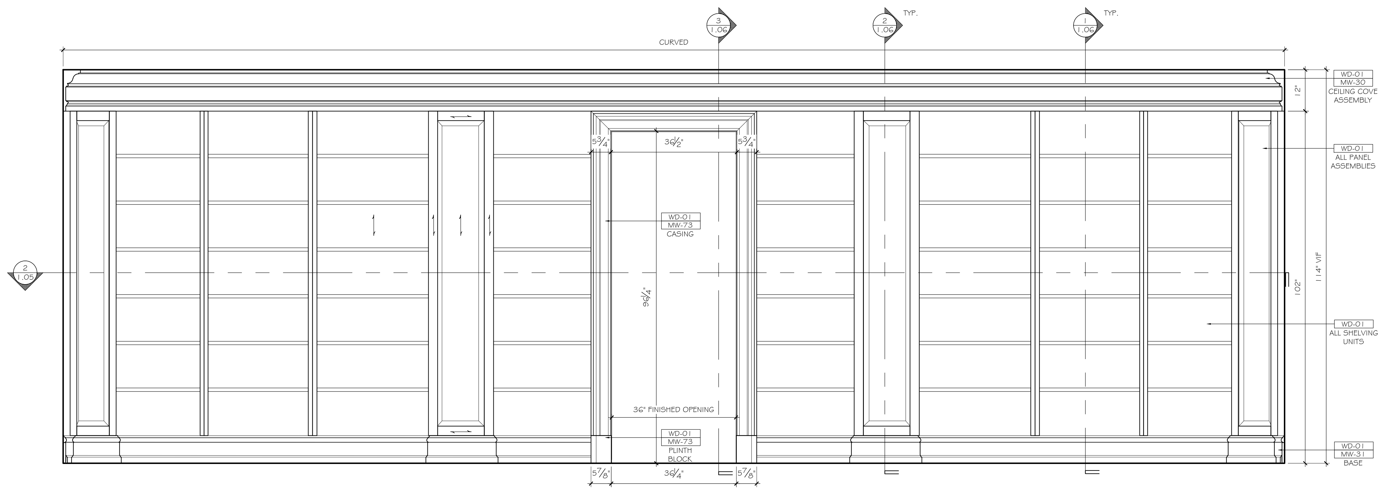
2 ELEVATION 1.03 SCALE: 3/4" = 12" ARCH. REF.: 3/A5.2
