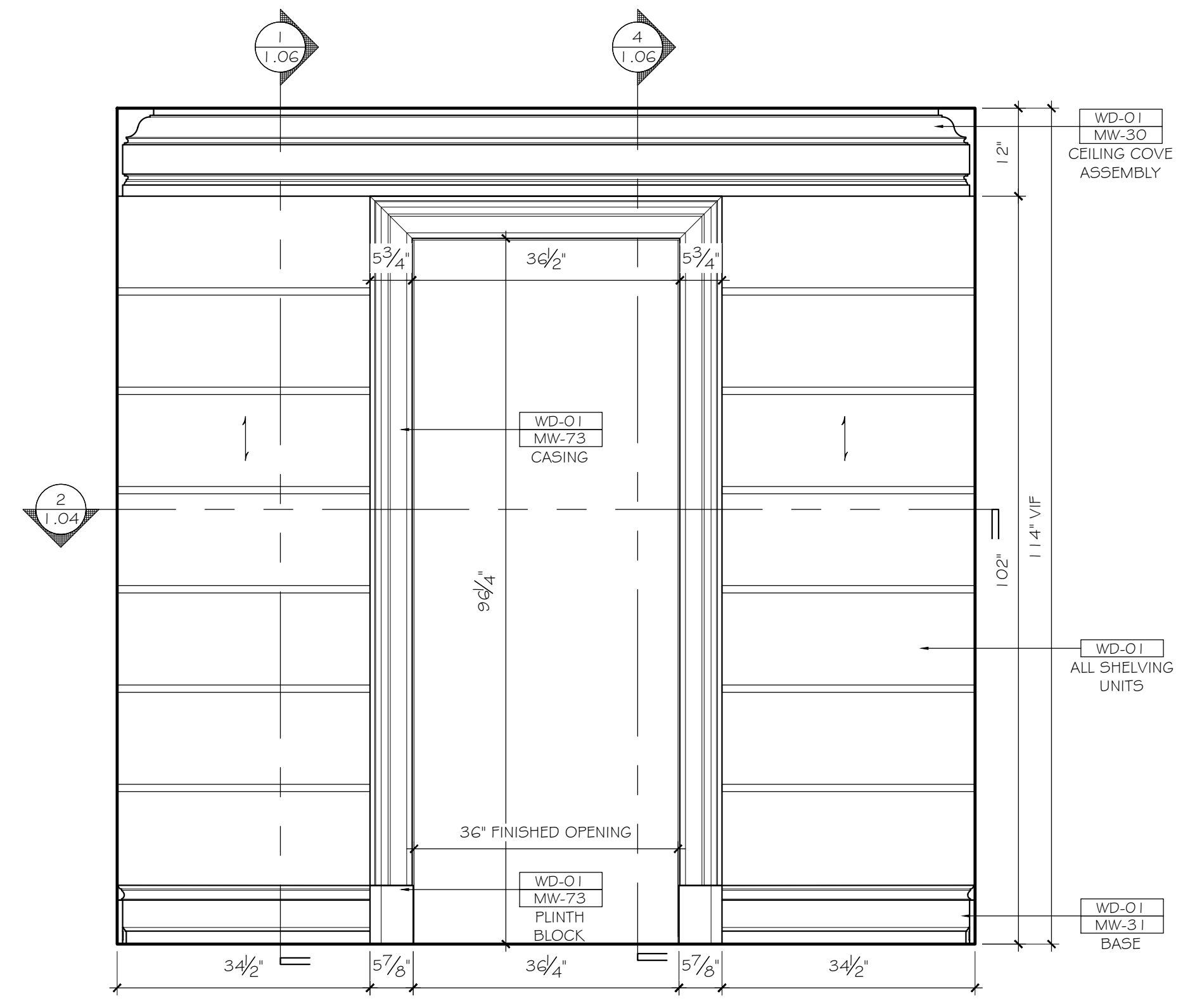
2 ELEVATION 1.02 SCALE: 3/4" = 12" ARCH. REF.: 4/A5.2
