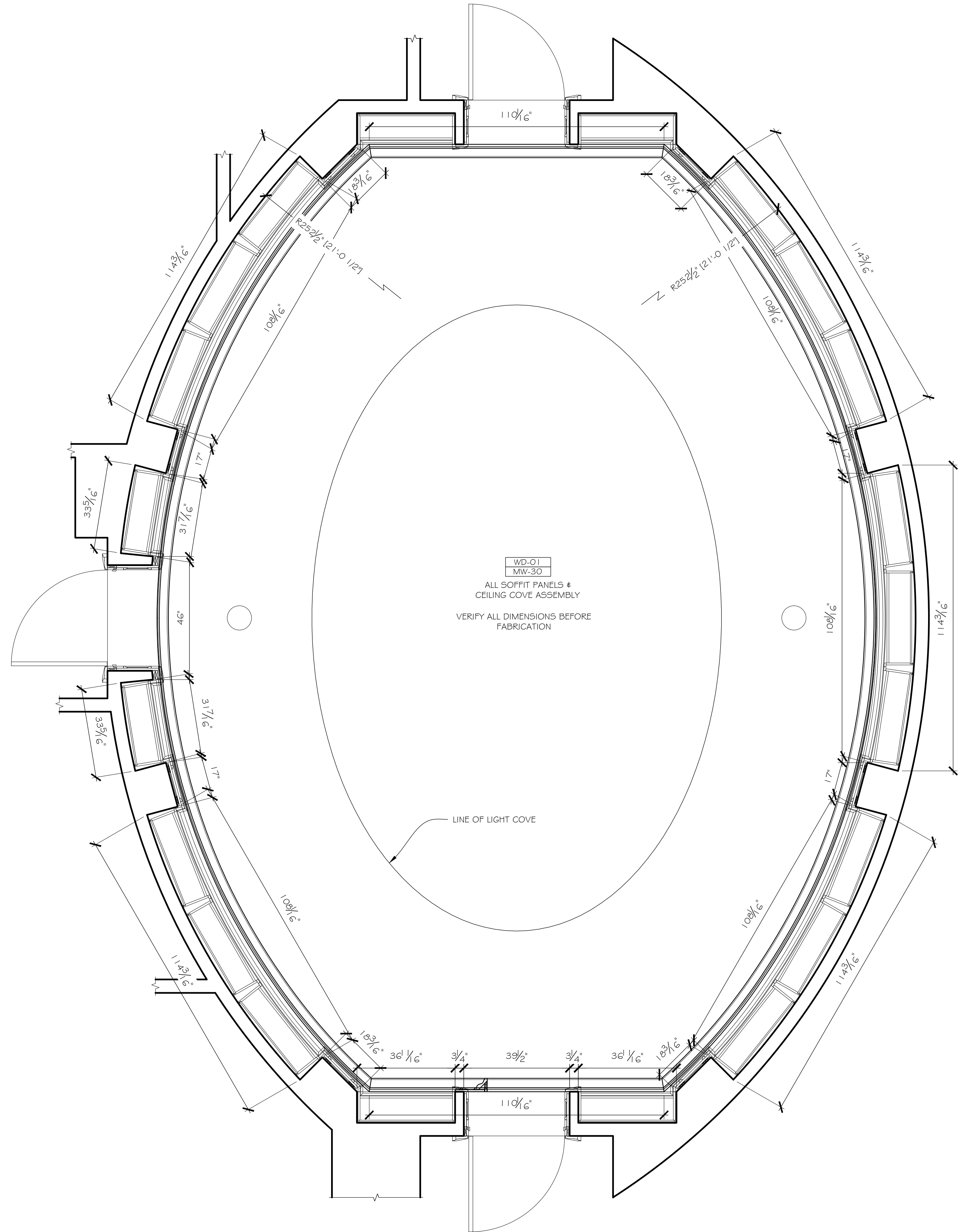
1 RCP 1.02 SCALE: 1/2" = 12" ARCH. REF.: NONE
