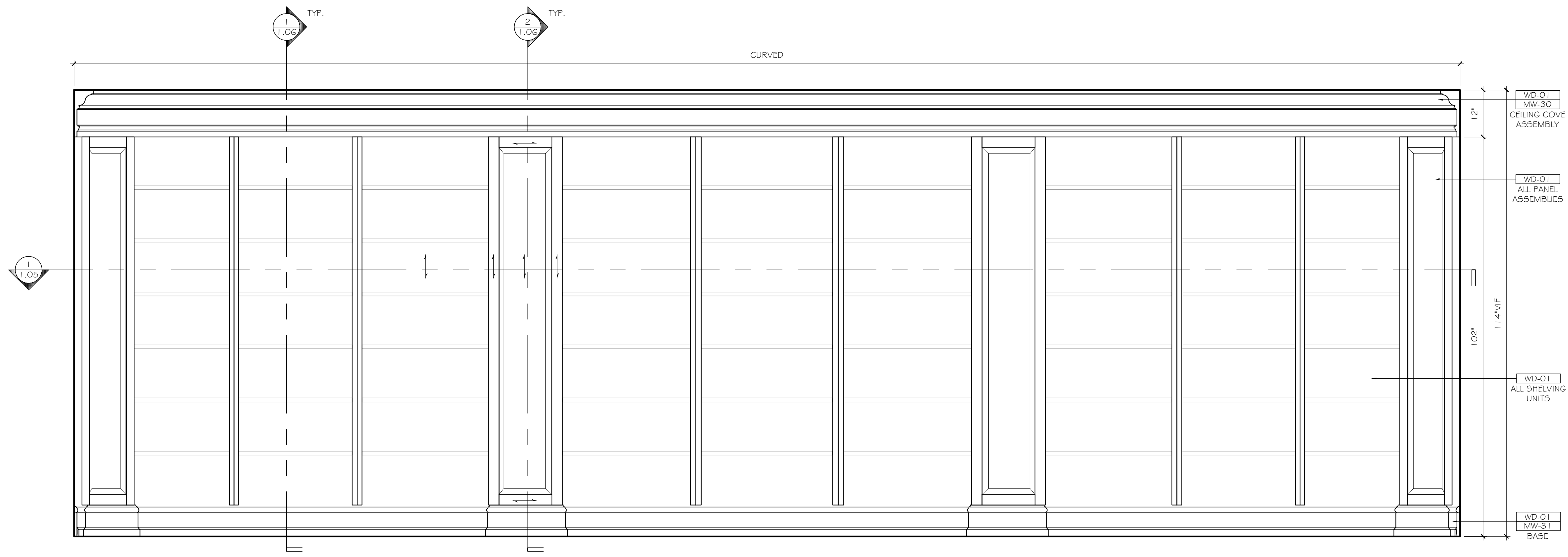
1 ELEVATION 1.03 SCALE: 3/4" = 12" ARCH. REF.: 5/A5.2
