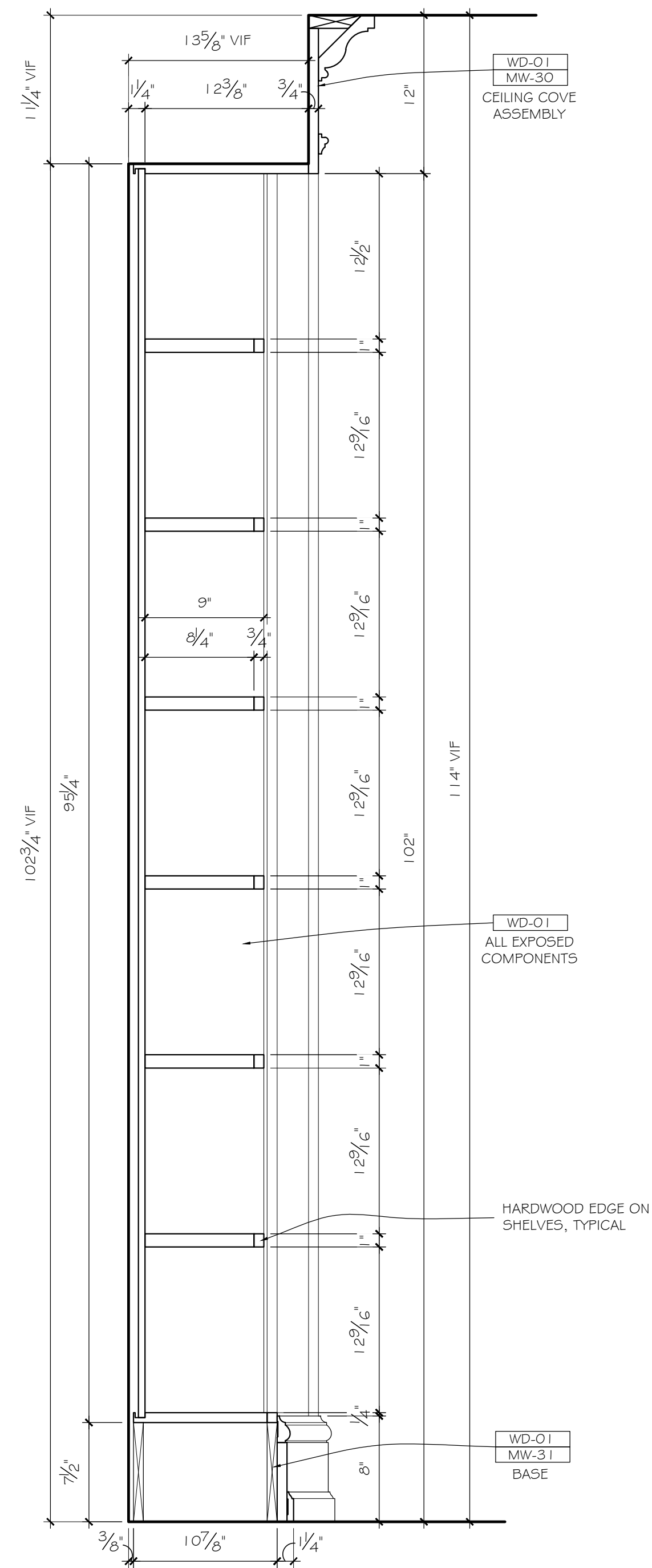
1 SECTION 1.06 SCALE: 1/2" = 12" ARCH. REF.: 3/A5.2.1
