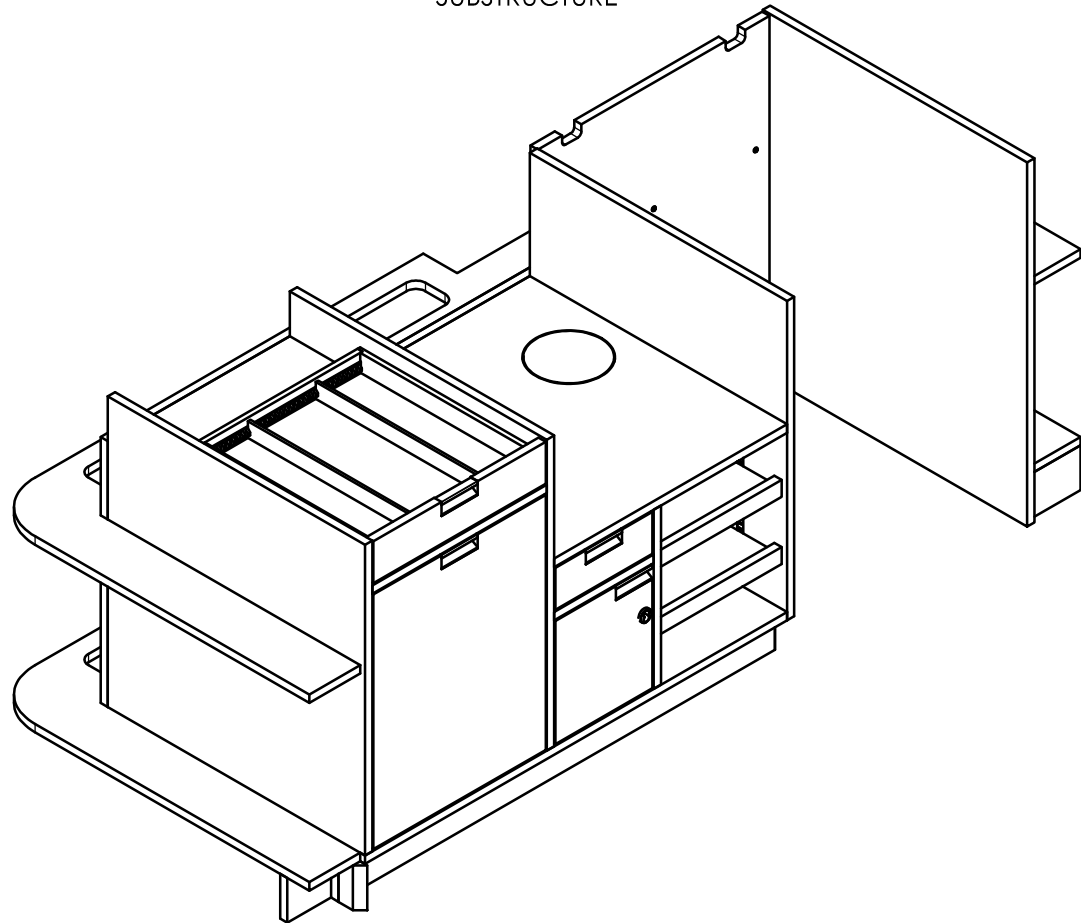
ISOMETRIC SUBSTRUCTURE
