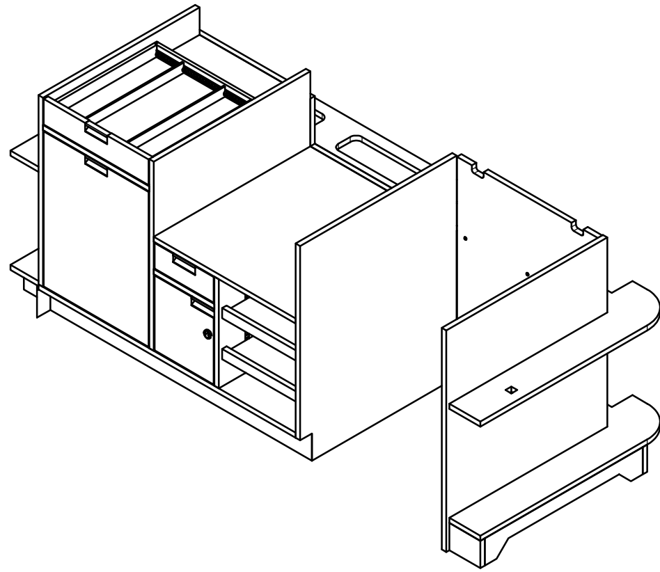
ISOMETRIC SUBSTRUCTURE
