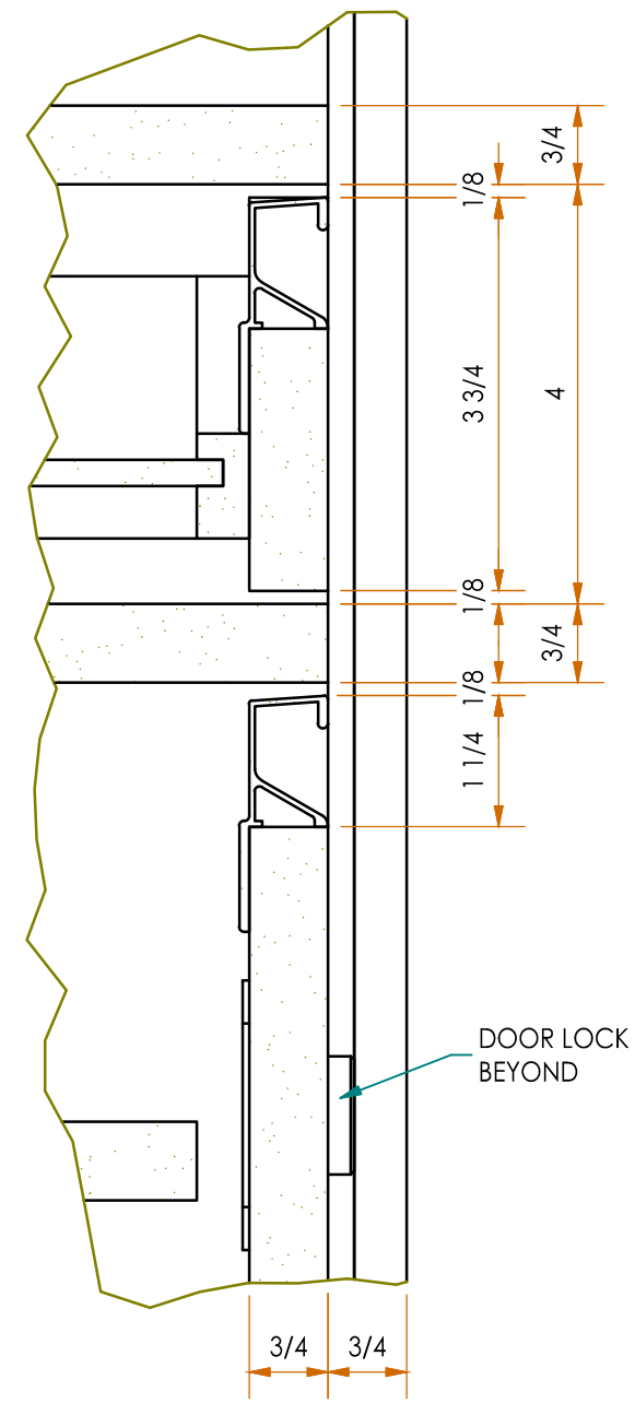
DETAIL 06
