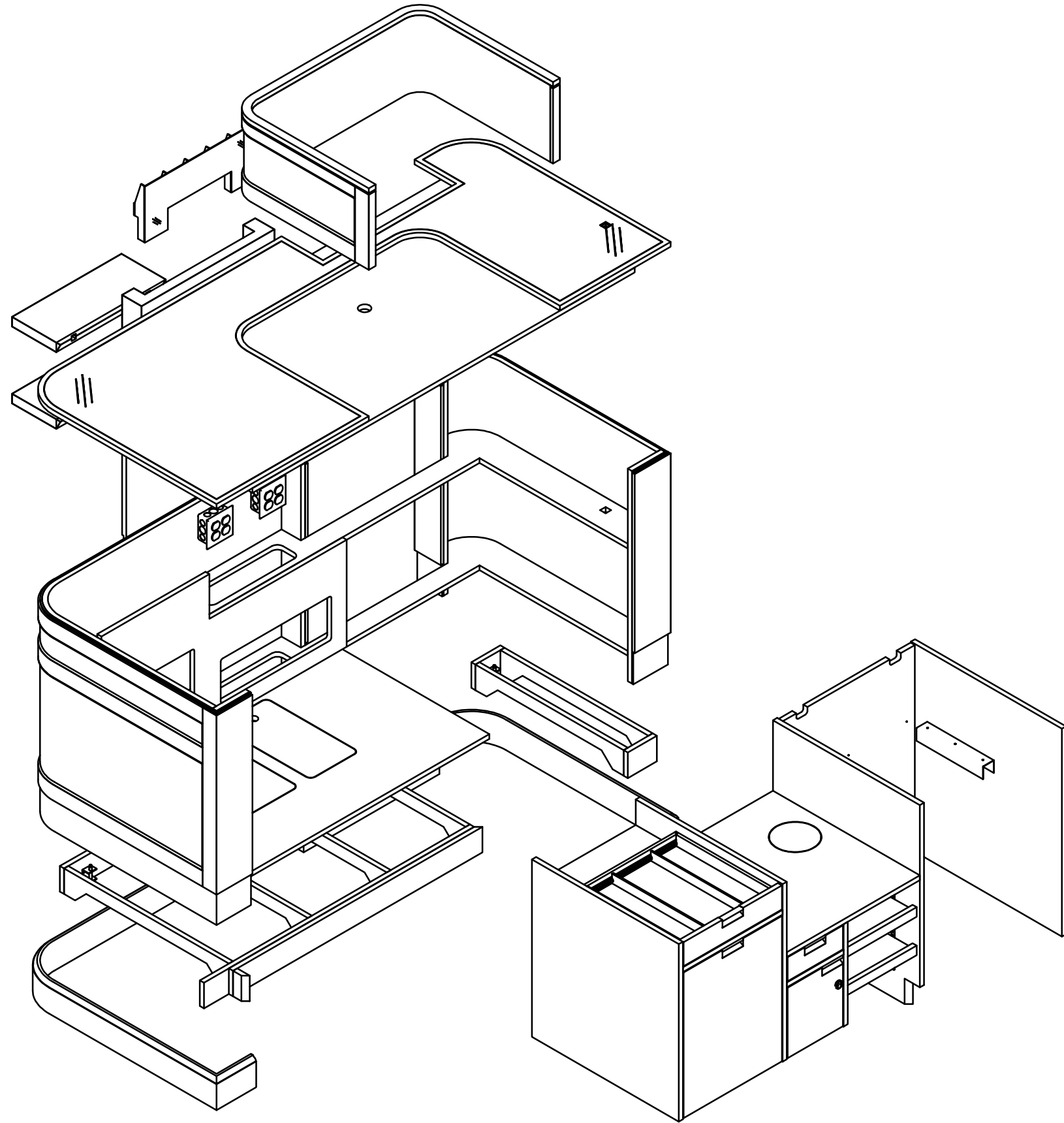
EXPLODED ISOMETRIC
