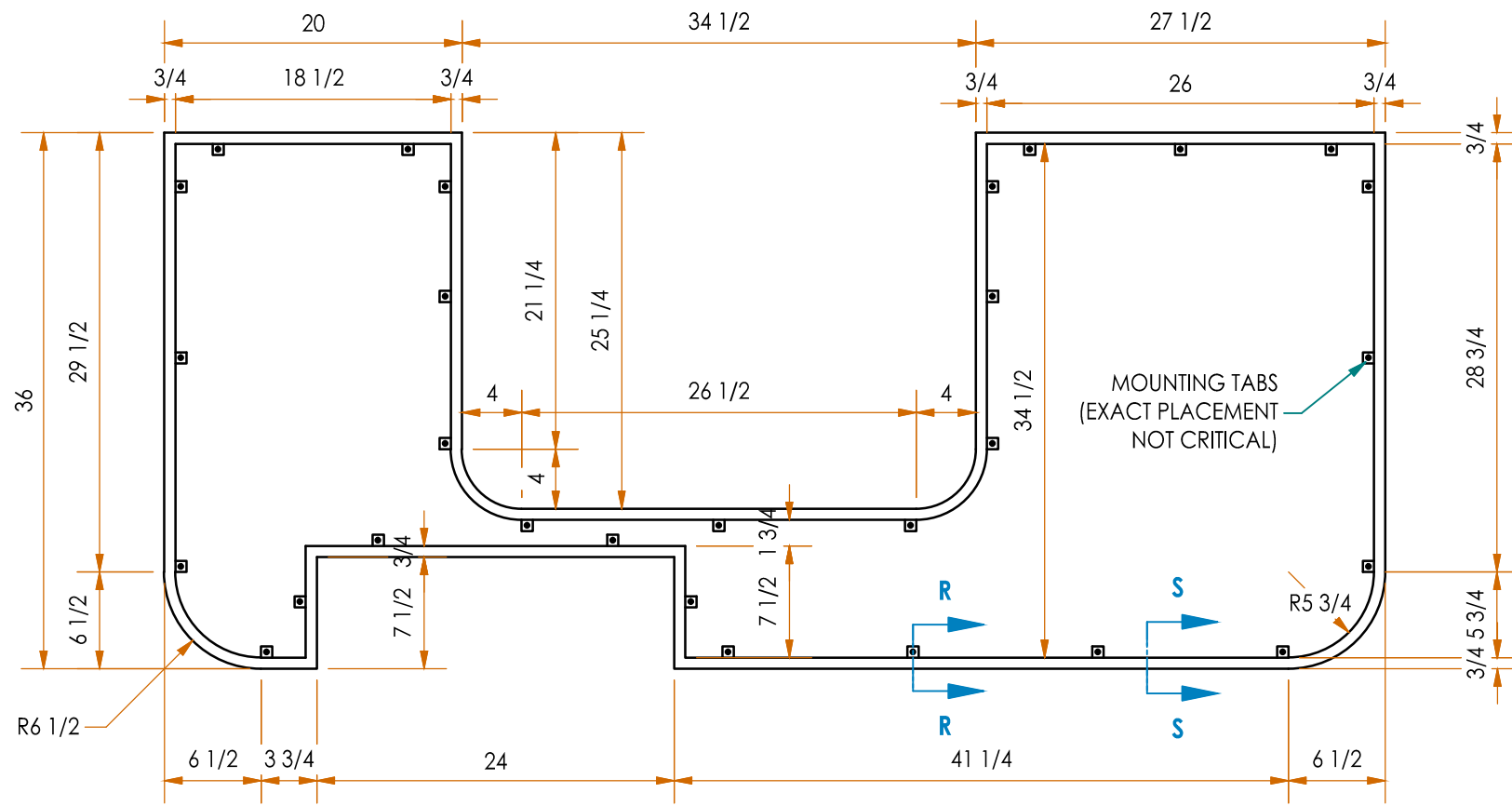
PLAN VIEW TOP; METAL PERIMETER
