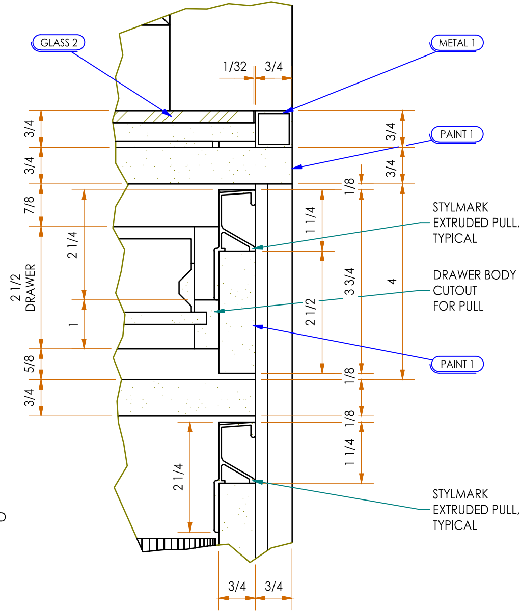
DETAIL 05
