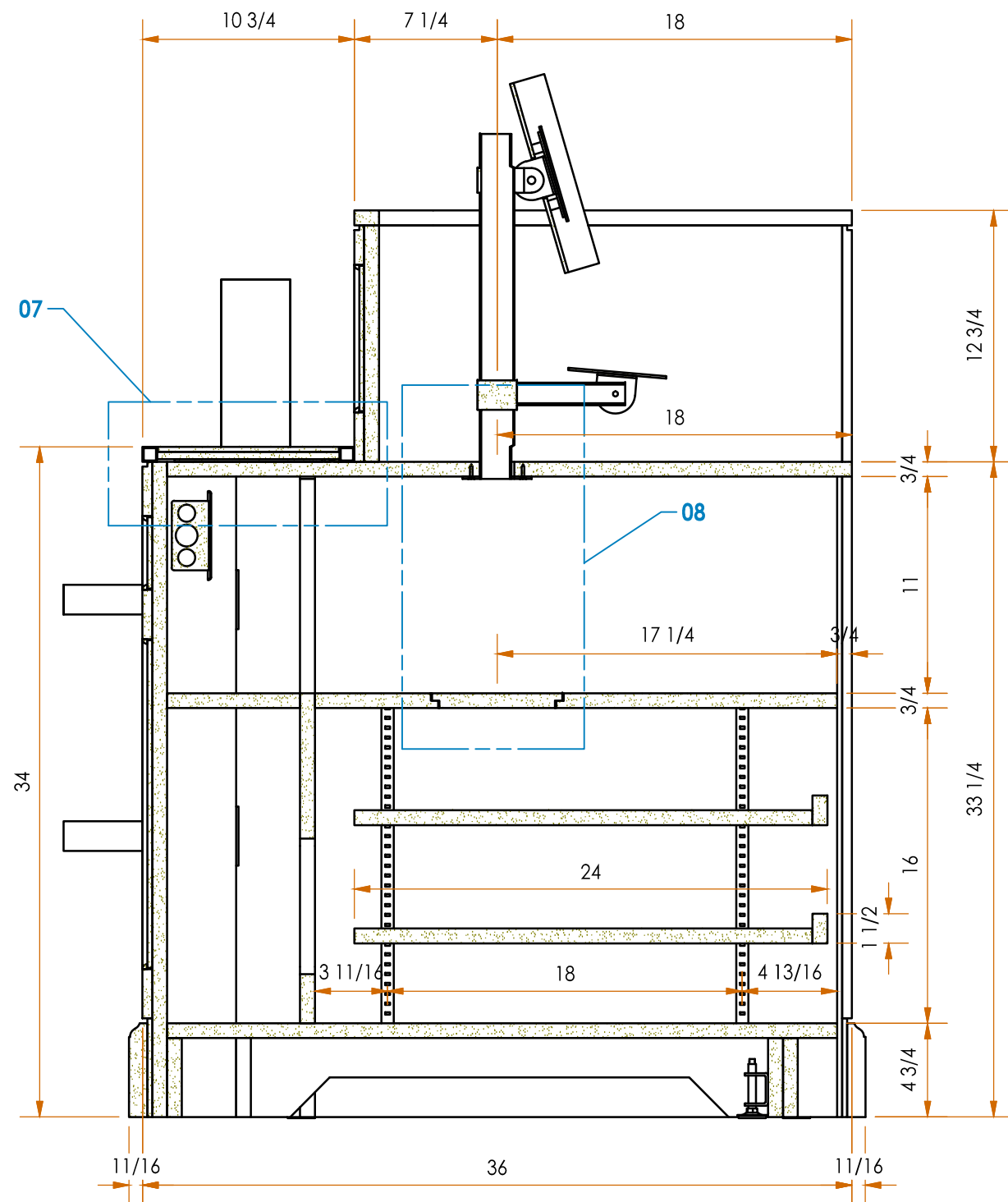
SECTION J-J
