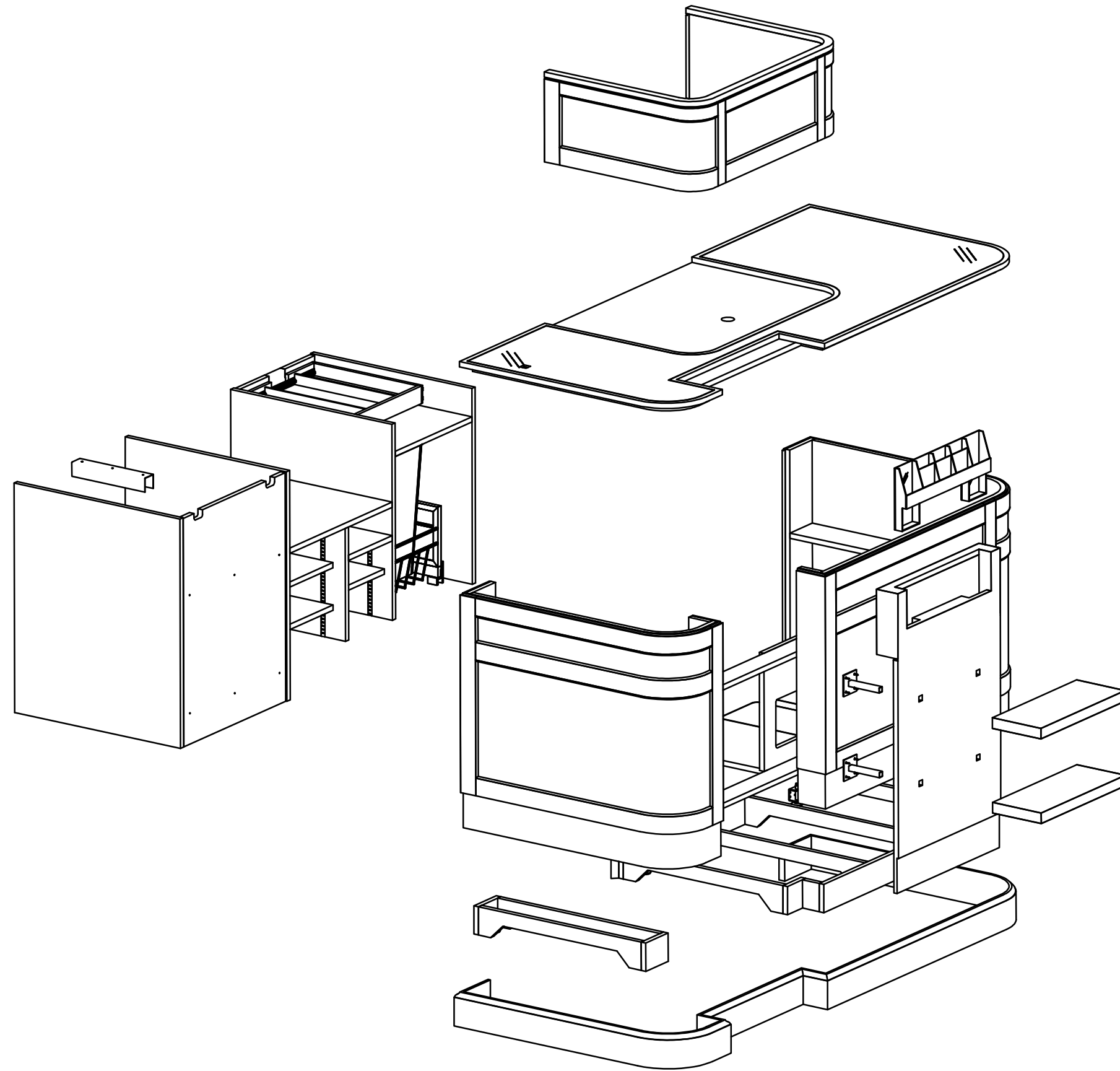
EXPLODED ISOMETRIC
