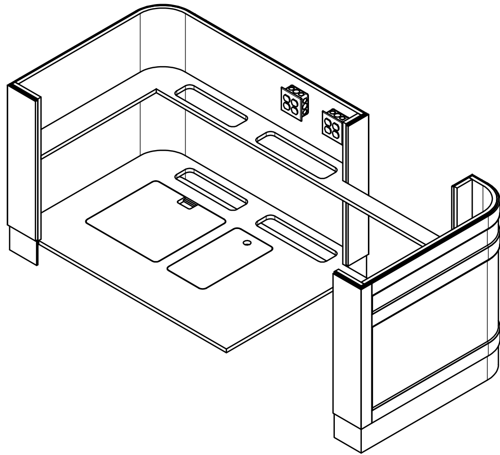
ISOMETRIC CARCASS
