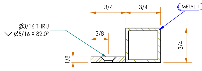
SECTION R-R
