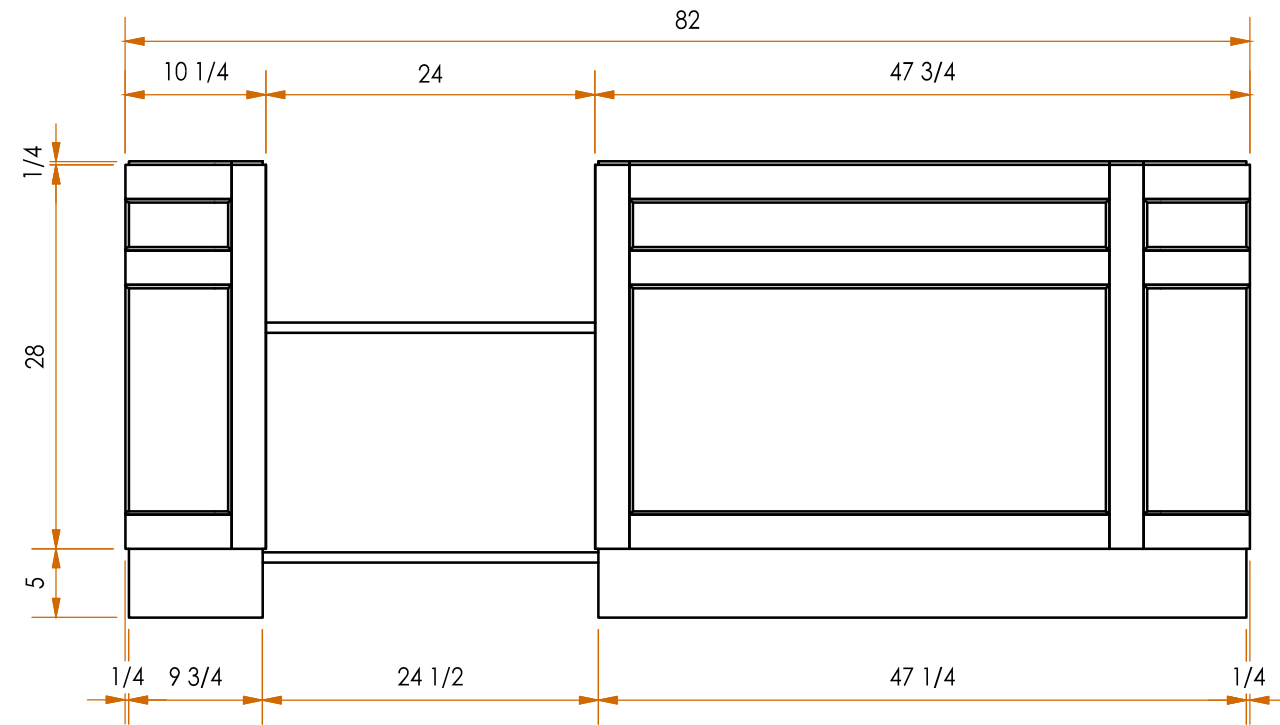
ELEVATION CARCASS; CUSTOMER SIDE
