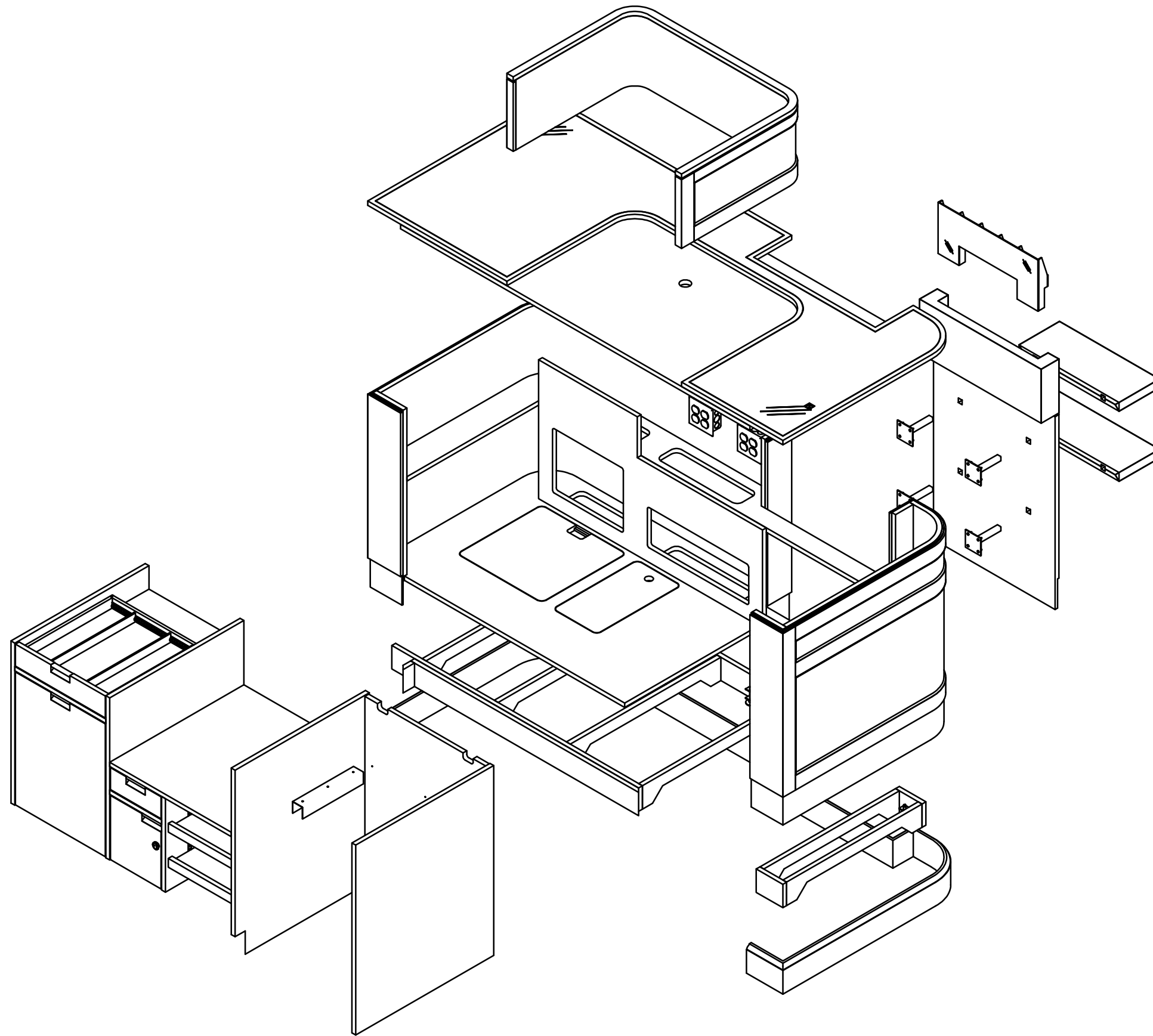
EXPLODED ISOMETRIC
