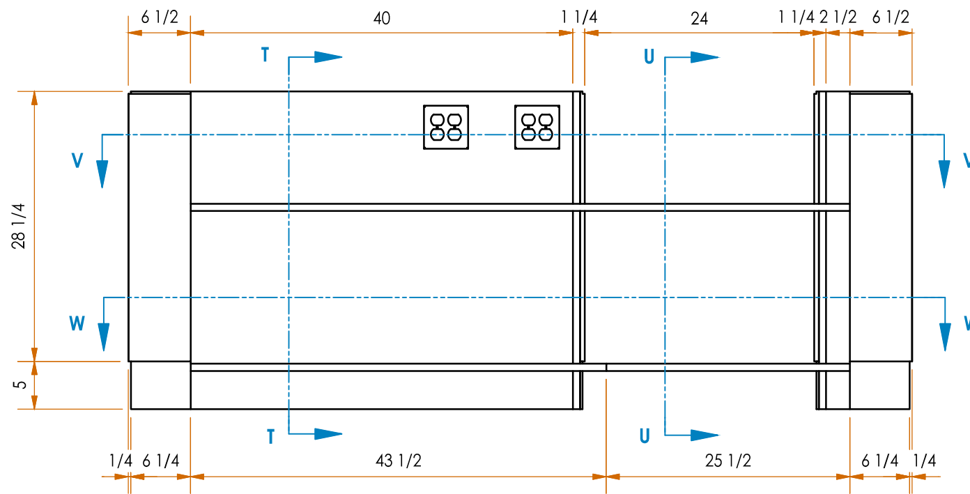
ELEVATION CARCASS; ASSOCIATE SIDE
