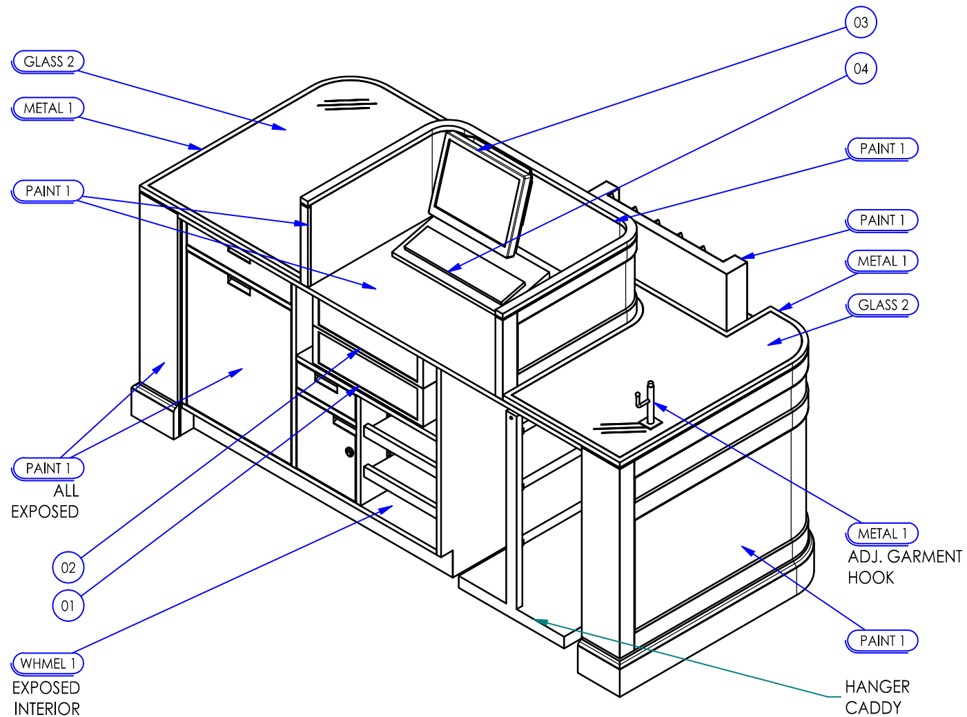
ISOMETRIC ASSOCIATE SIDE
