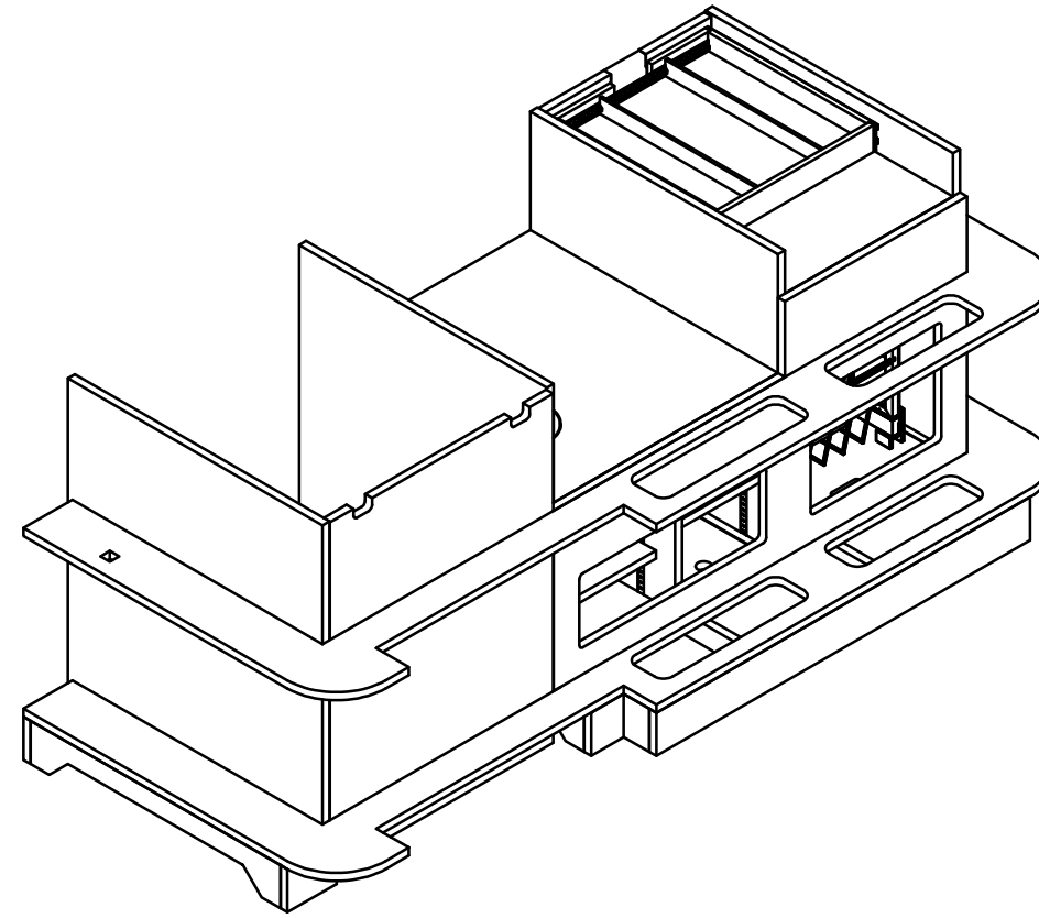
ISOMETRIC SUBSTRUCTURE
