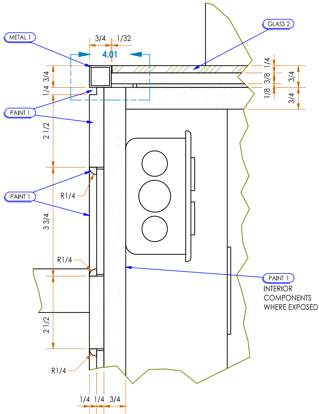
DETAIL 04
