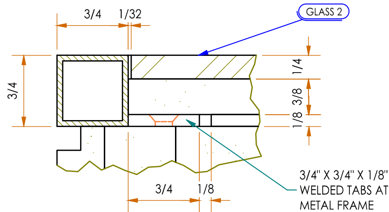
DETAIL 4.01
