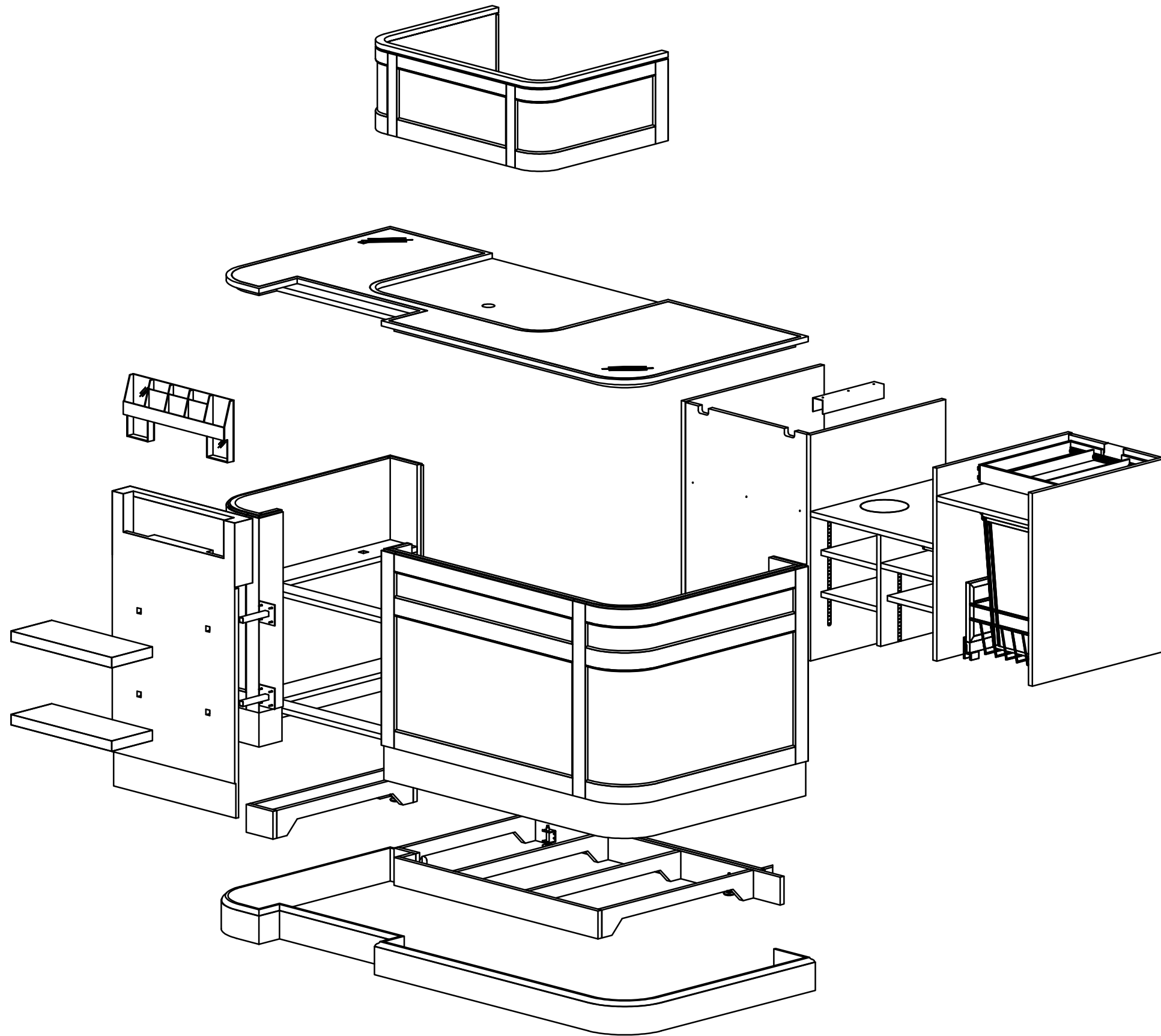
EXPLODED ISOMETRIC
