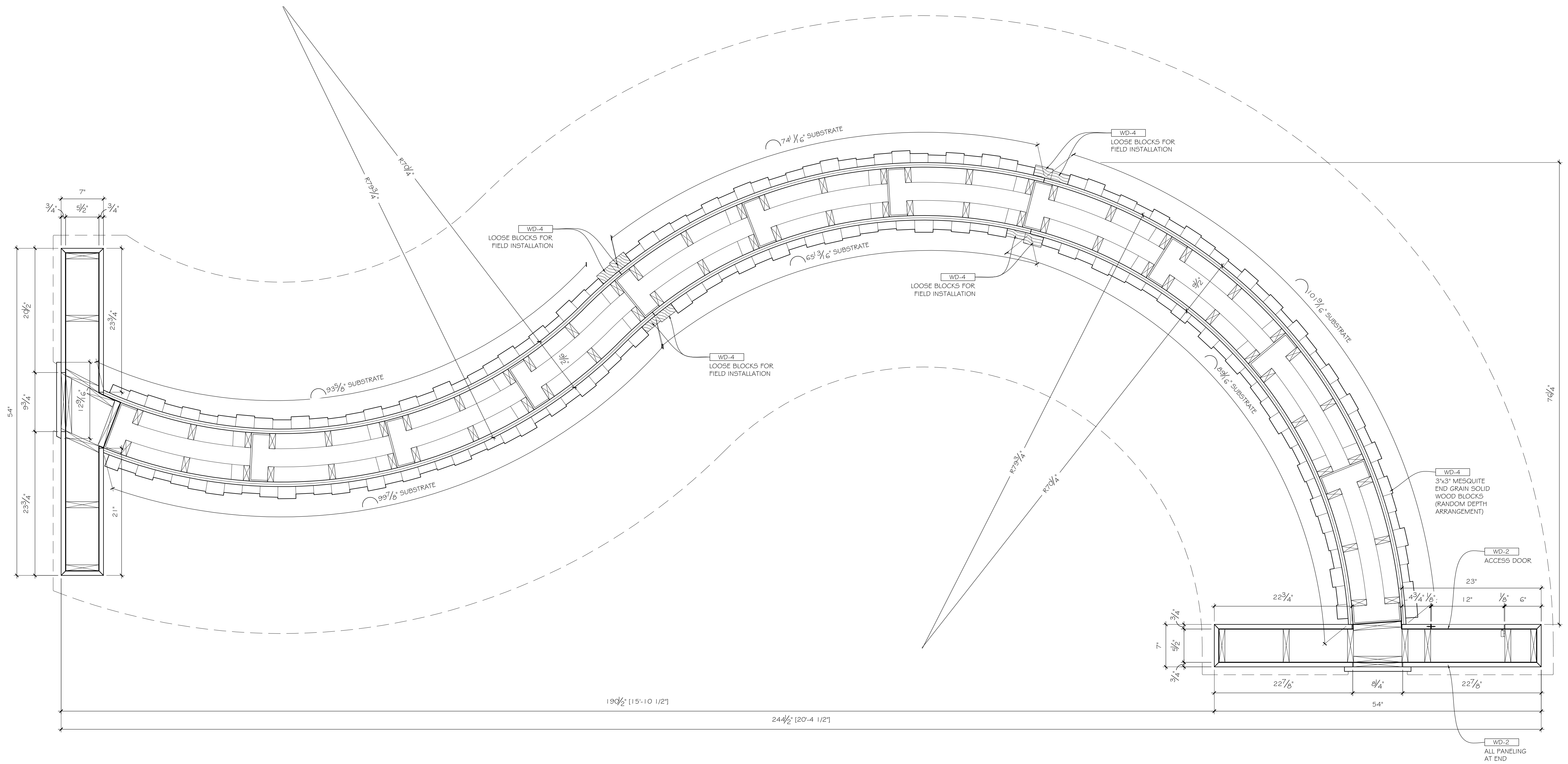
1 PLAN SECTION: 3.47 SCALE: 1-1/2"=1' ARCH. REF.: NONE
