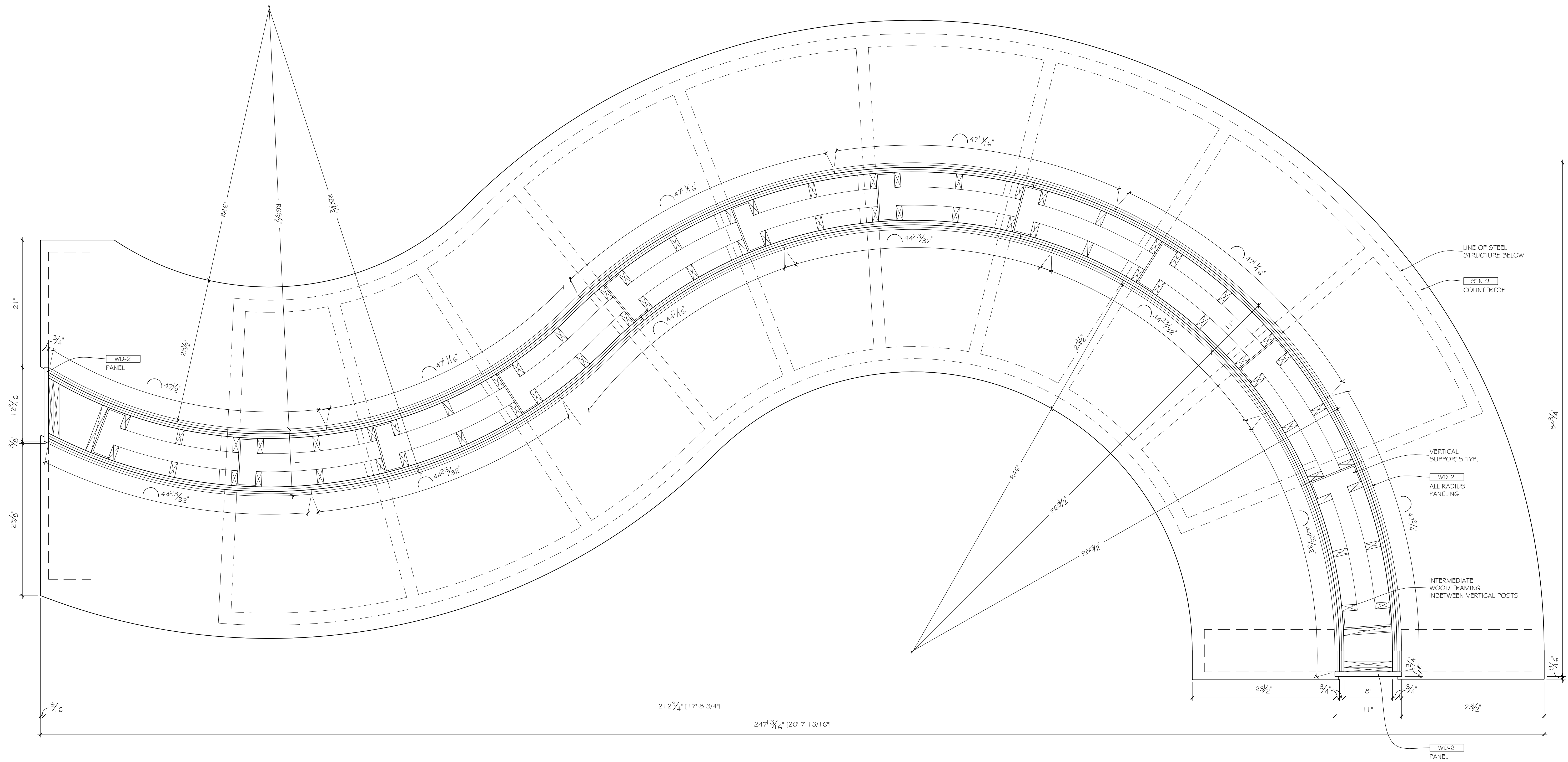
1 PLAN SECTION: 3.46 SCALE: 1-1/2"=12" ARCH. REF.: NONE
