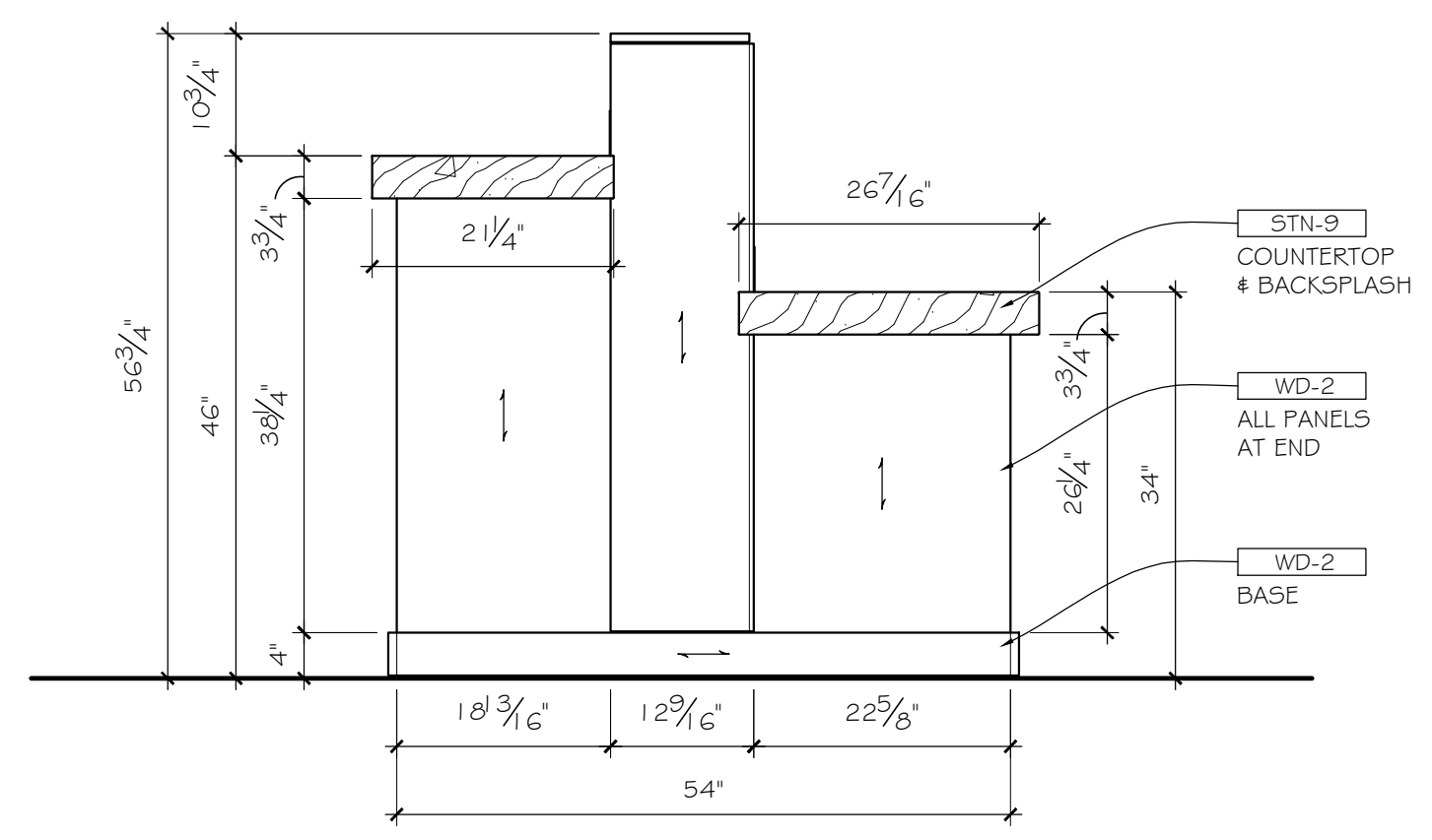
2 ELEVATION: 3.42 SCALE: 3/4" = 1' ARCH. REF.: 6/A-565-O
