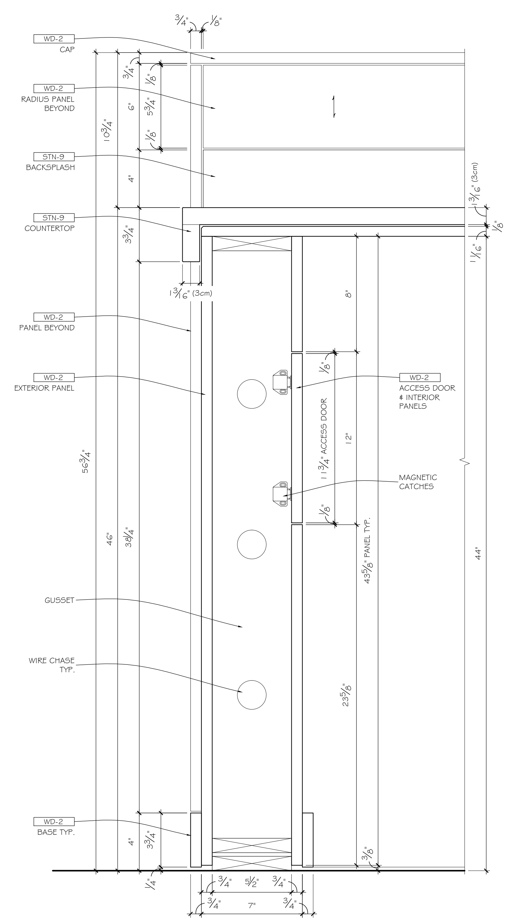
3 SECTION: 3.43 SCALE: 3"=12" ARCH. REF.: 1/OA-565-0
