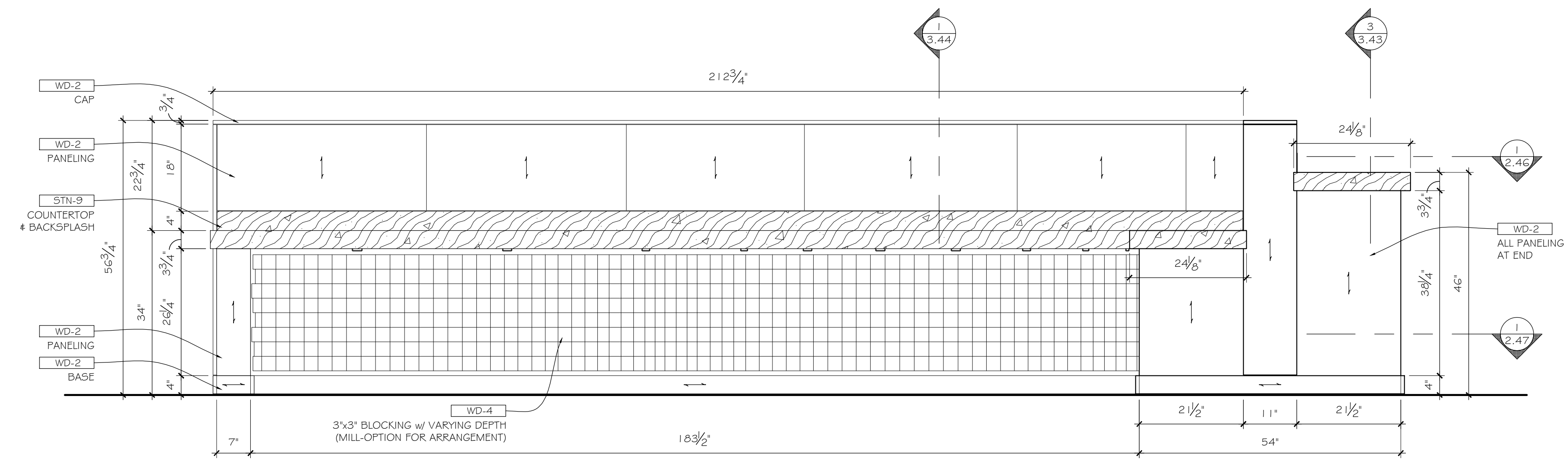
2 ELEVATION: 3.43 SCALE: 3/4"=12" ARCH. REF.: 5/A-565-0
