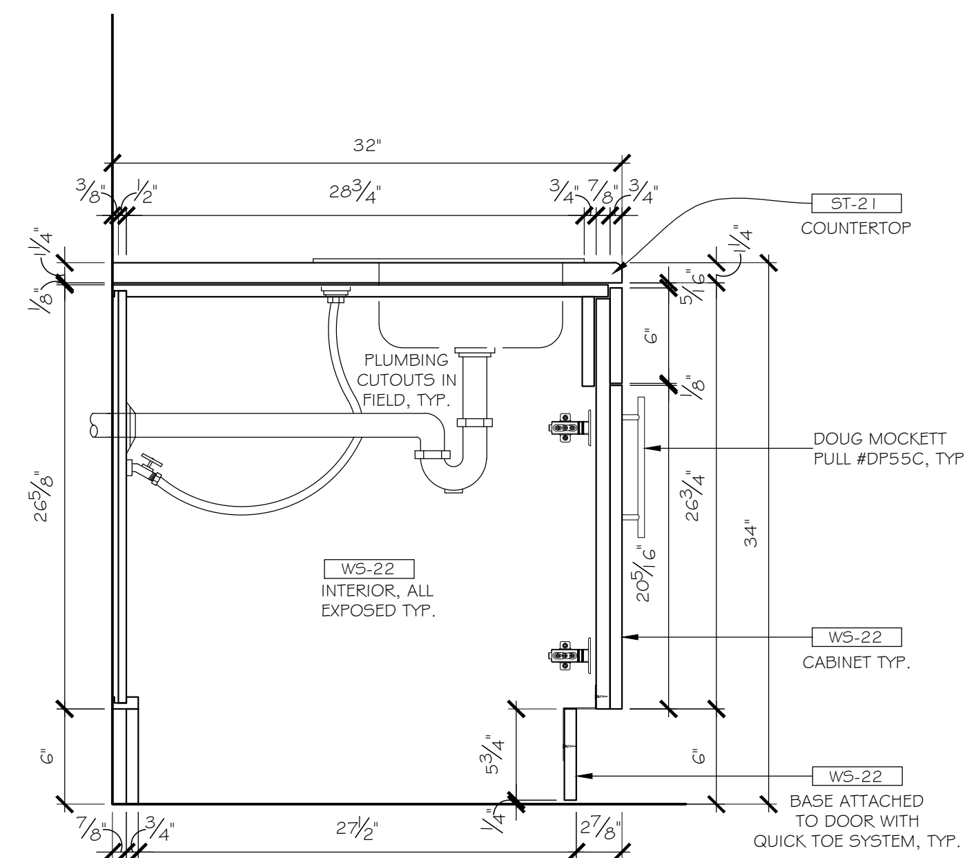
2 SECTION 2.05 SCALE: 1 1/2" = 12" ARCH. REF.: 9/A-573
