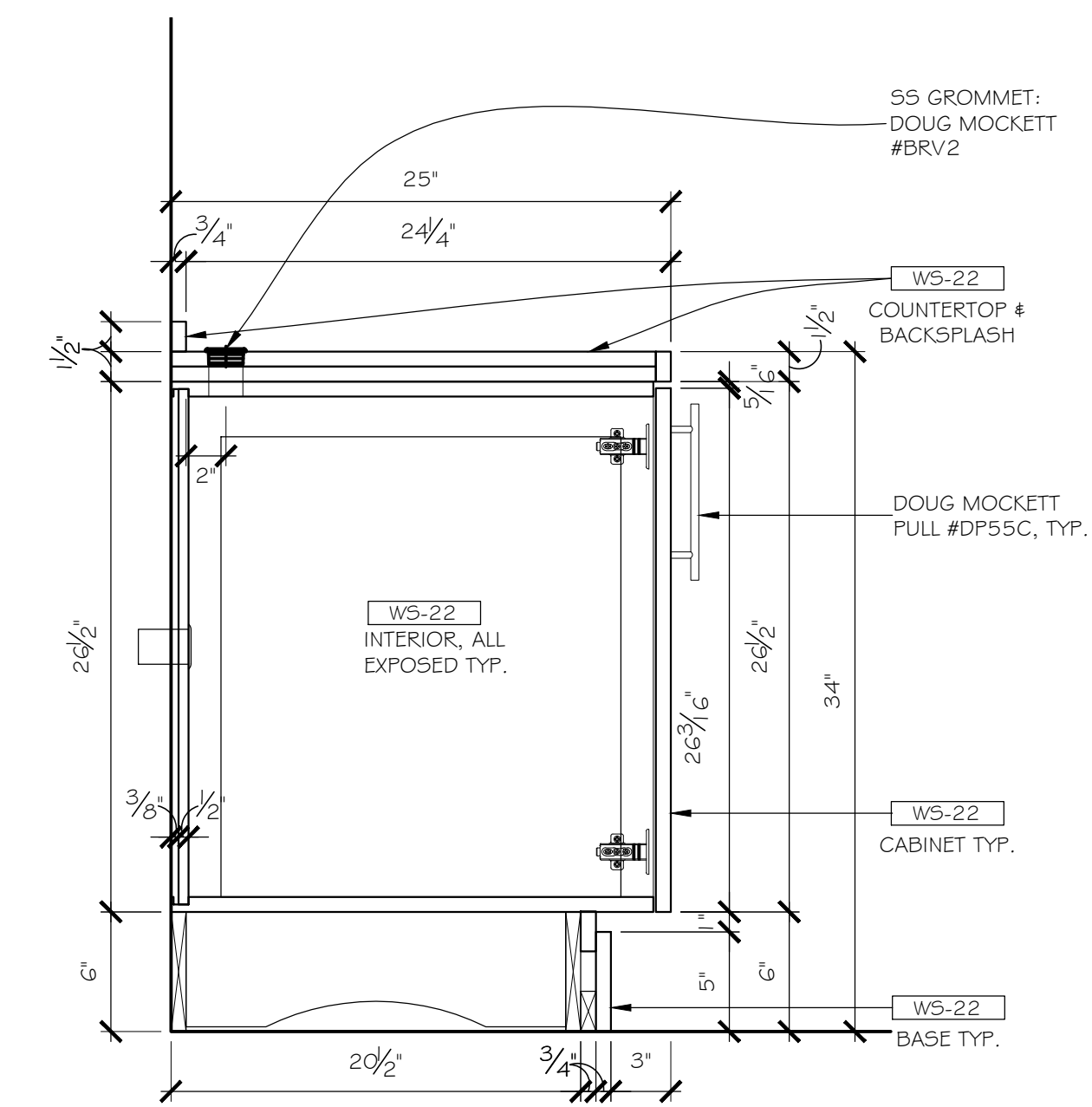
3 SECTION 2.05 SCALE: 1 1/2" = 12" ARCH. REF.: 8/A-573
