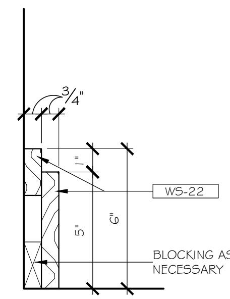
6 SECTION 2.05 SCALE: 3" = 12" ARCH. REF.: 15/A-573
