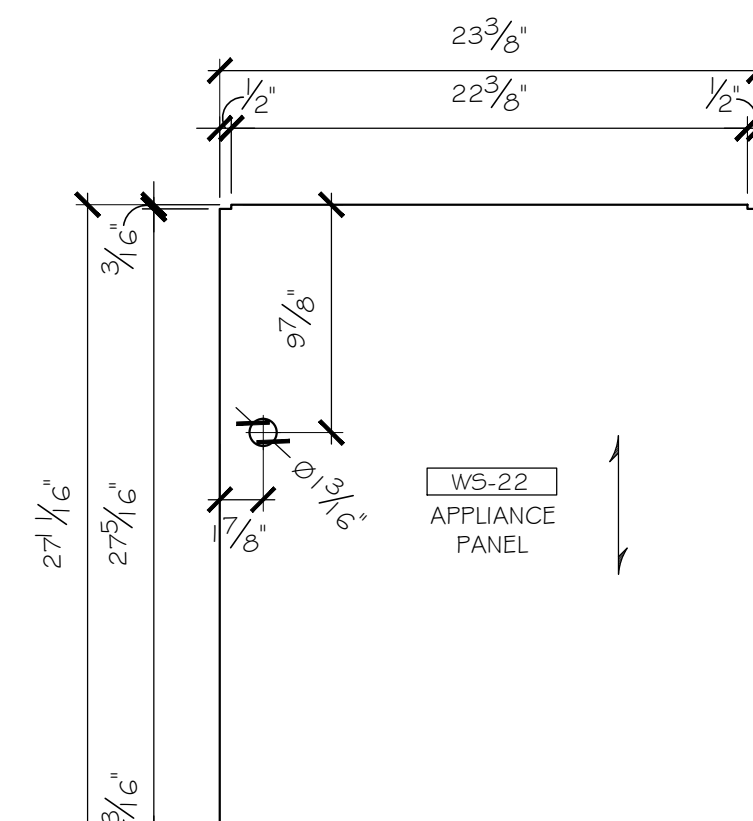
5 DETAIL: REFRIGERATOR PANEL 2.05 SCALE: 1 1/2" = 12" ARCH. REF.: NONE
