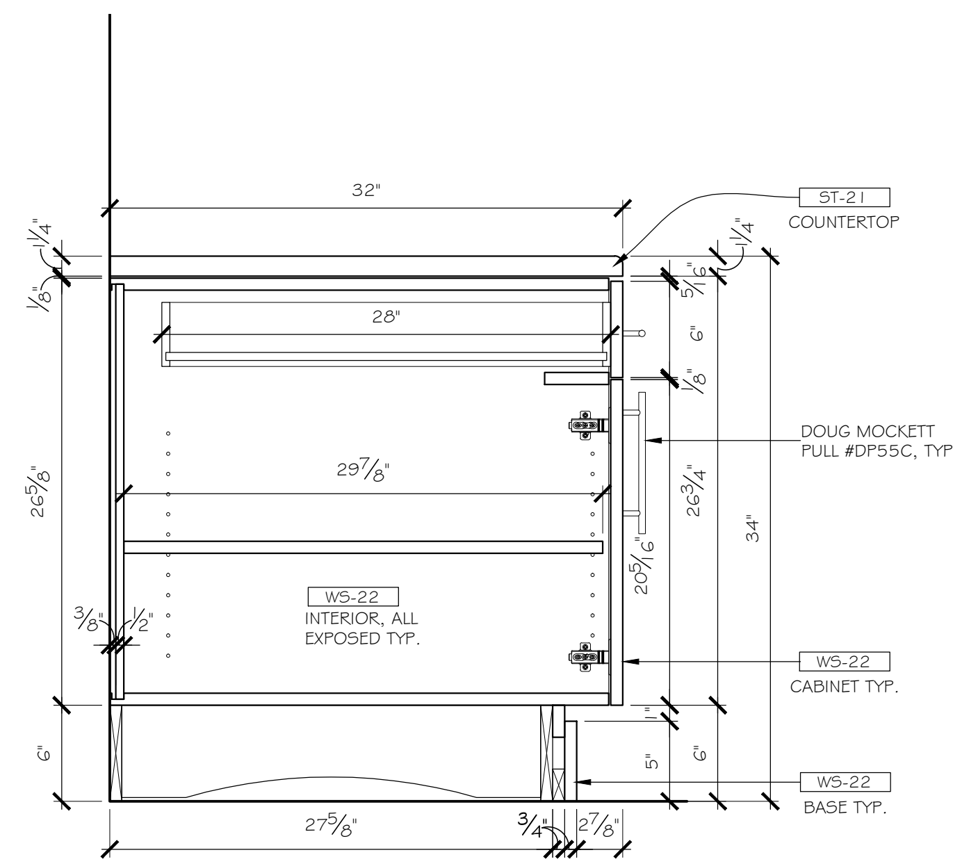
1 SECTION 2.05 SCALE: 1 1/2" = 12" ARCH. REF.: 3/A-573
