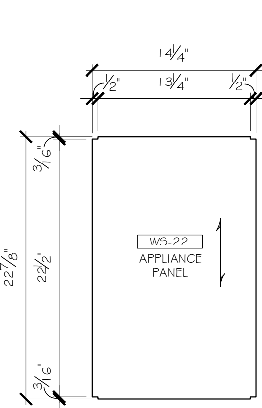
4 DETAIL: FREEZER PANEL 2.05 SCALE: 1 1/2" = 12" ARCH. REF.: NONE
