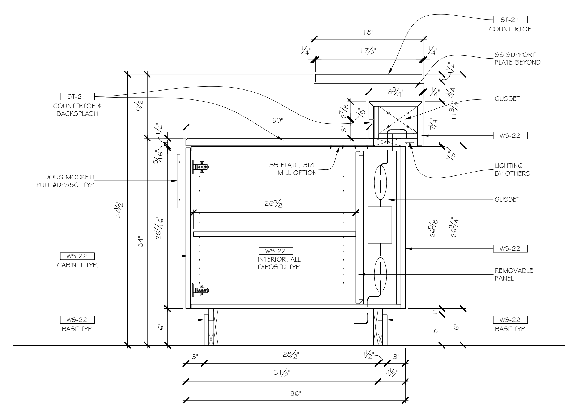
7 SECTION 2.05 SCALE: 1 1/2" = 12" ARCH. REF.: 5/A-573
