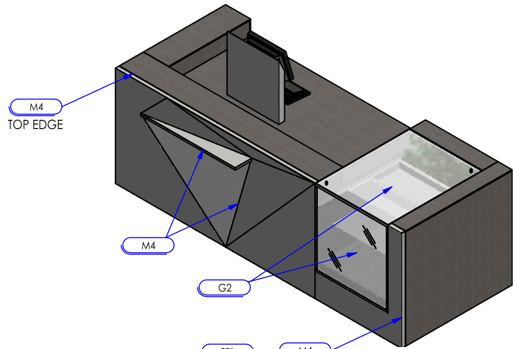
ISOMETRIC CUSTOMER SIDE - ADA SHELF IN
