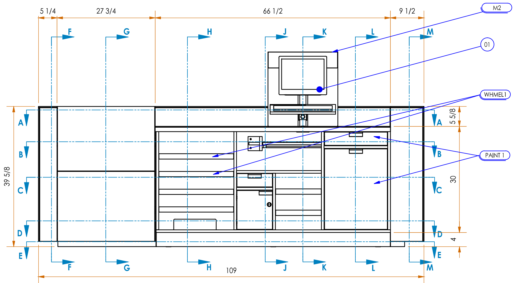
ELEVATION CLERK SIDE
