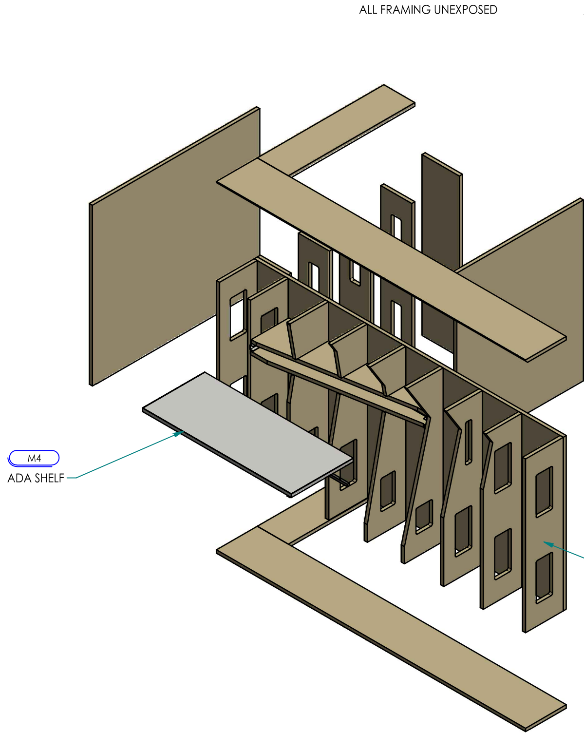
EXPLODED ISOMETRIC FRAMING
