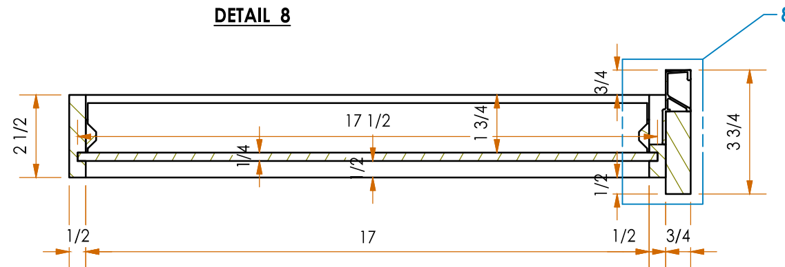
SECTION U-U
