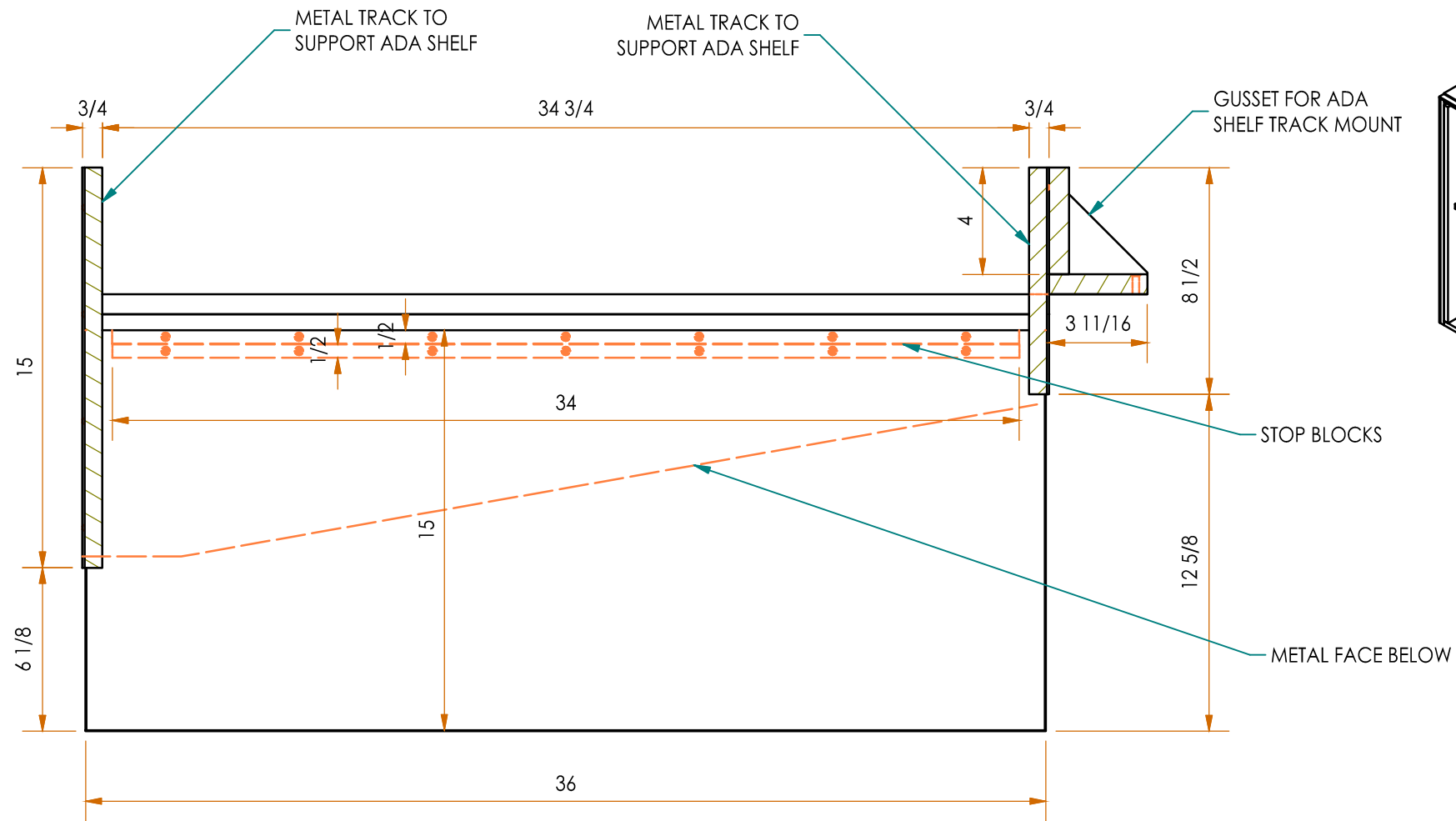
PLAN VIEW ADA SHELF
