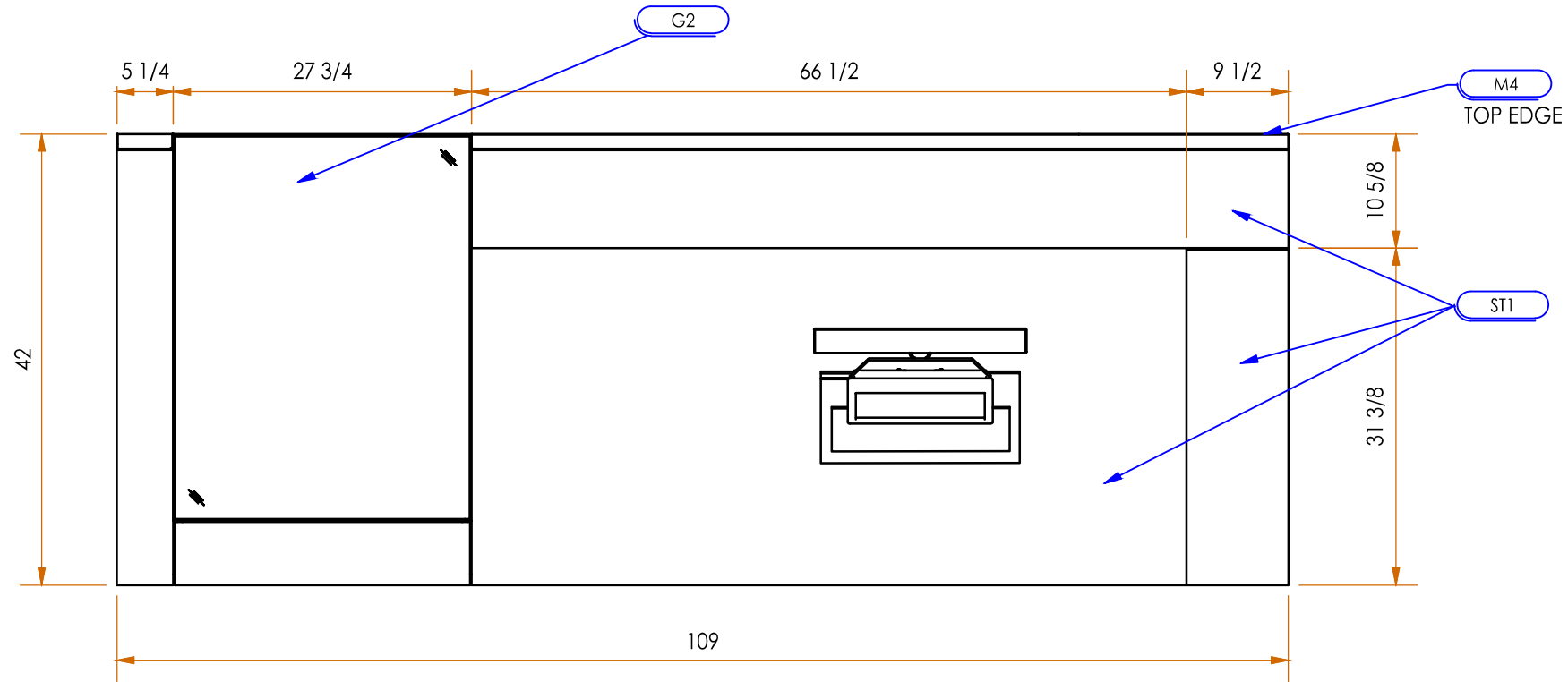
PLAN VIEW
