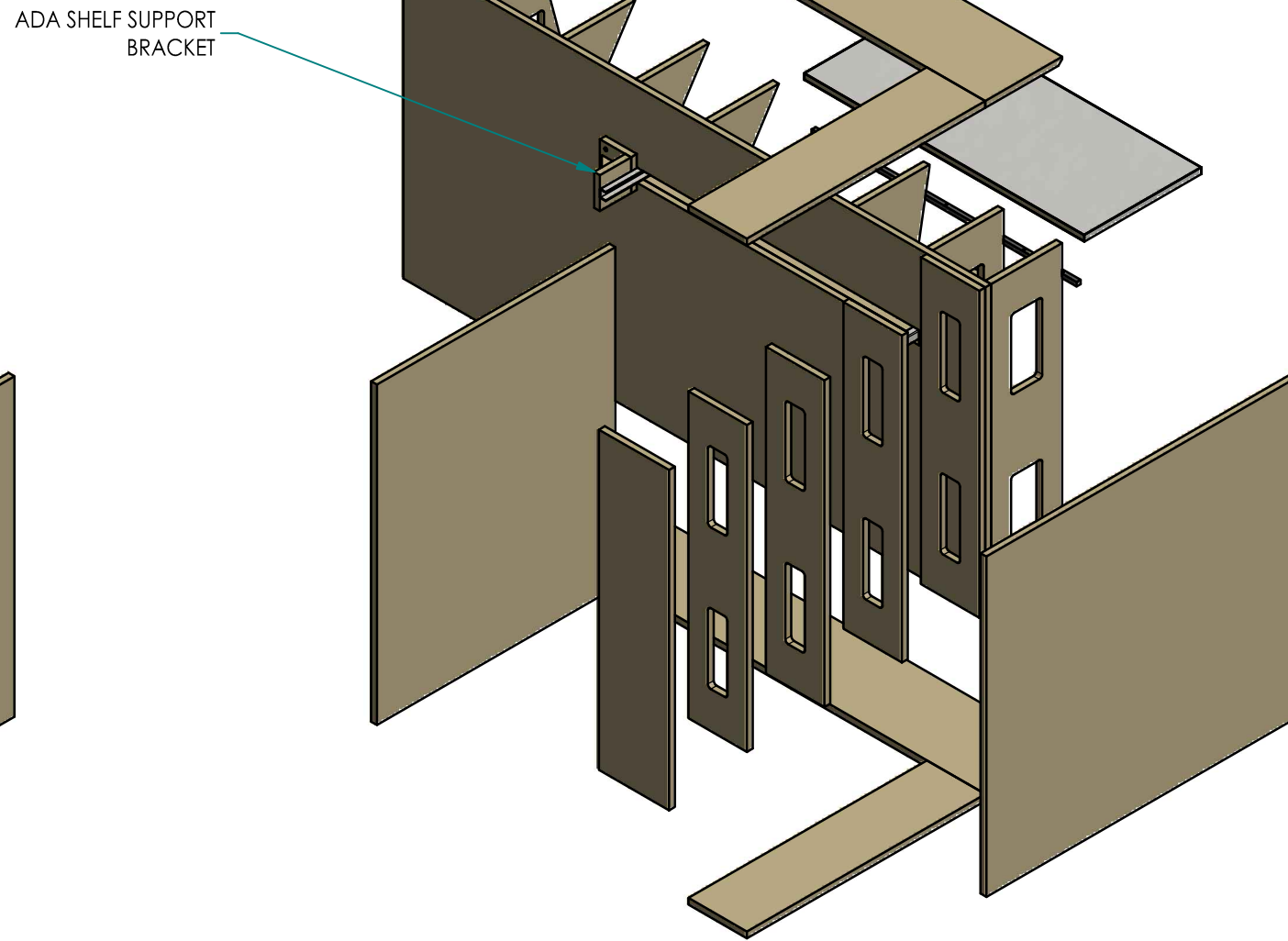
EXPLODED ISOMETRIC FRAMING
