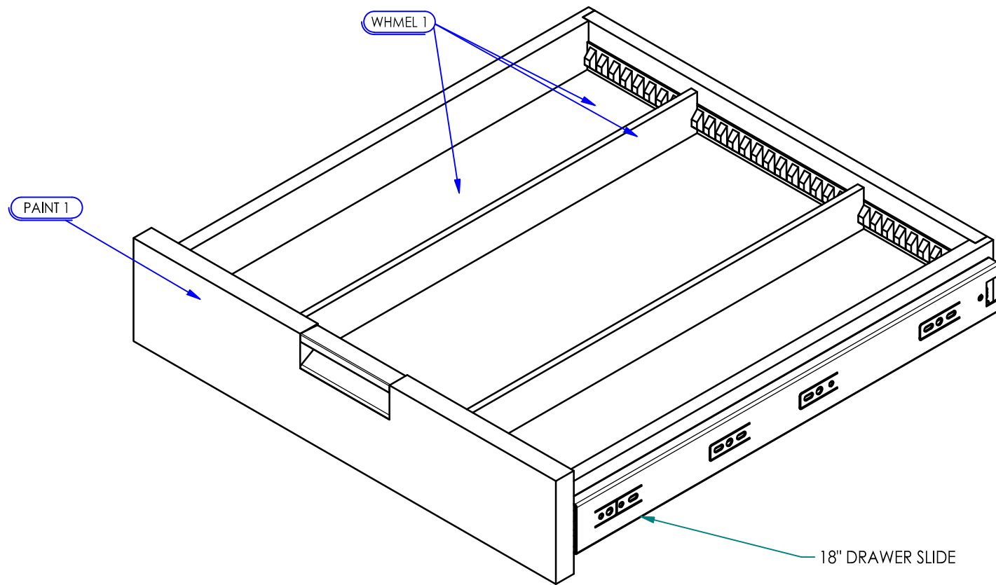
ISOMETRIC DRAWER
