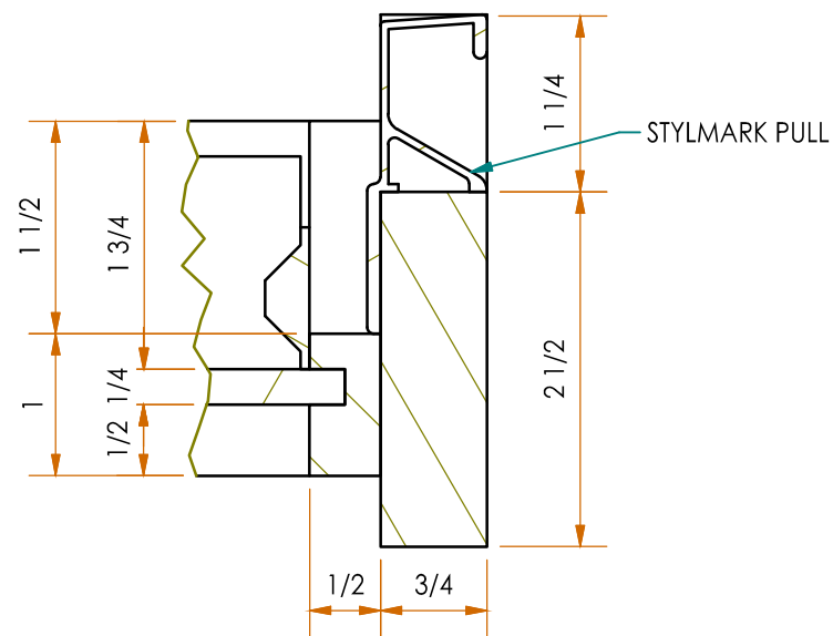
DETAIL 8
