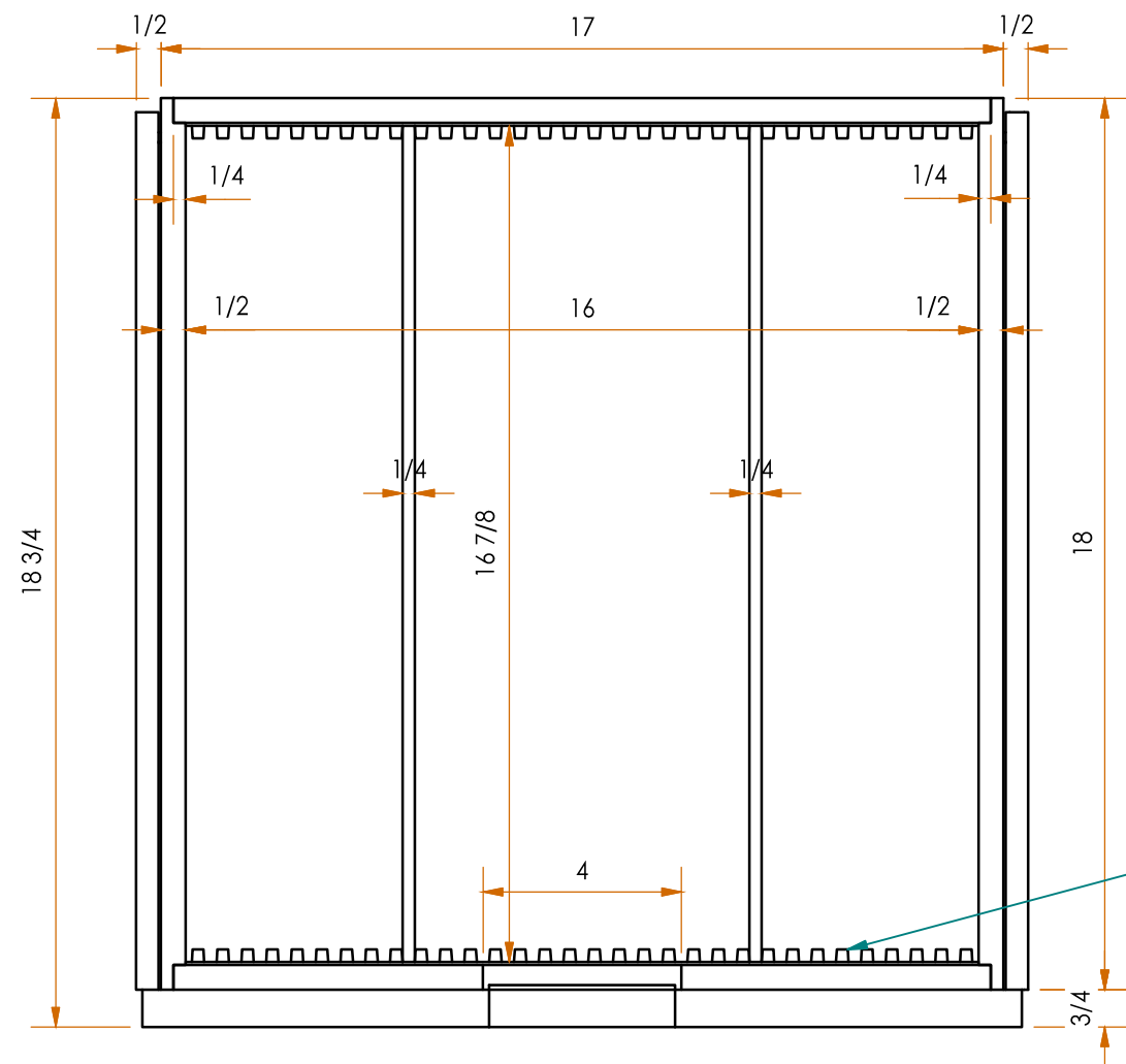
PLAN VIEW
