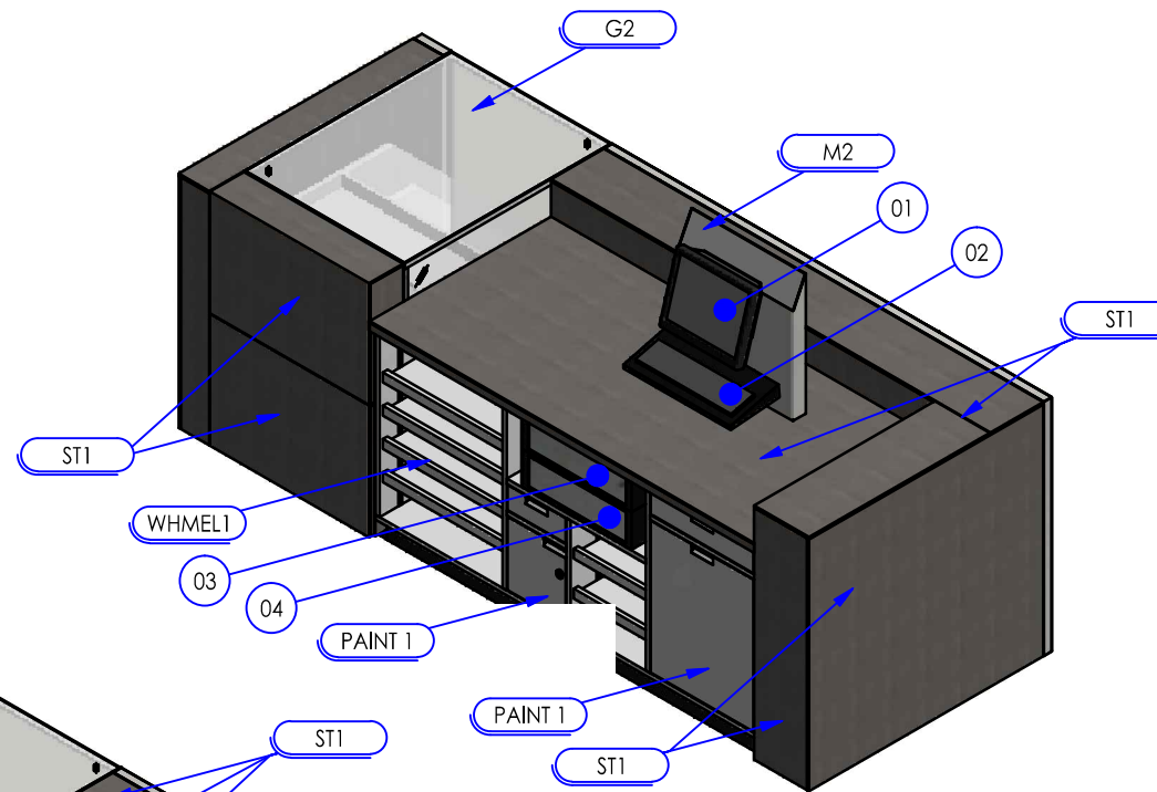
ISOMETRIC CLERK SIDE - DRAWERS IN
